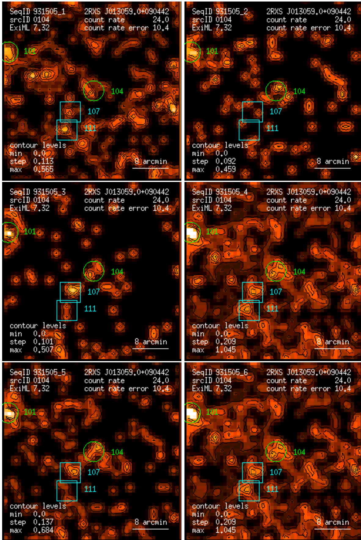
Figure 104: RASS 931505: detection 0104: band rate images, Gaussian filter: (1) PSPC channels 11 – 41, (2) 52 – 90, (3) 91 – 201, (4) 11 – 235, (5) 52 – 201, (6) 11 – 201. Broad band rates in counts/ks. Band rate contour levels in counts/ks/arcmin 2 .
