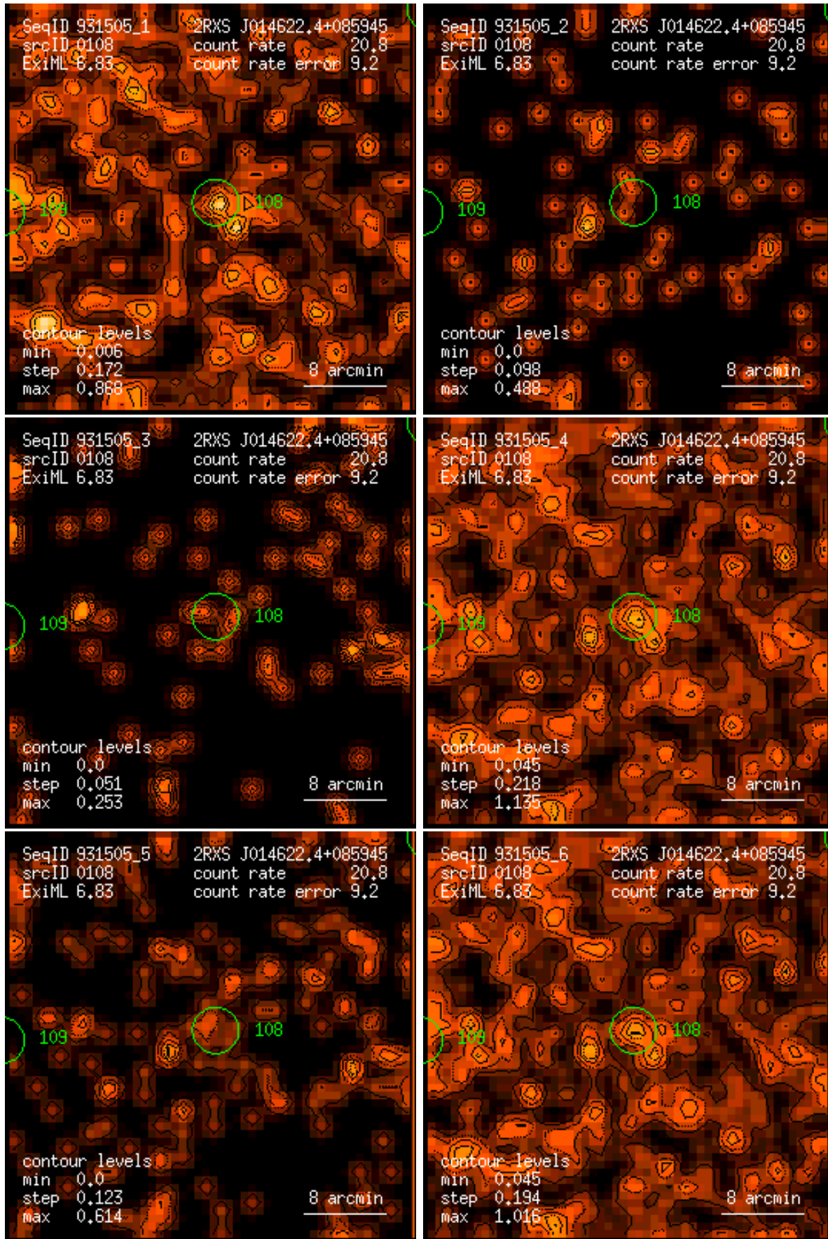
Figure 108: RASS 931505: detection 0108: band rate images, Gaussian filter: (1) PSPC channels 11 – 41, (2) 52 – 90, (3) 91 – 201, (4) 11 – 235, (5) 52 – 201, (6) 11 – 201. Broad band rates in counts/ks. Band rate contour levels in counts/ks/arcmin 2 .
