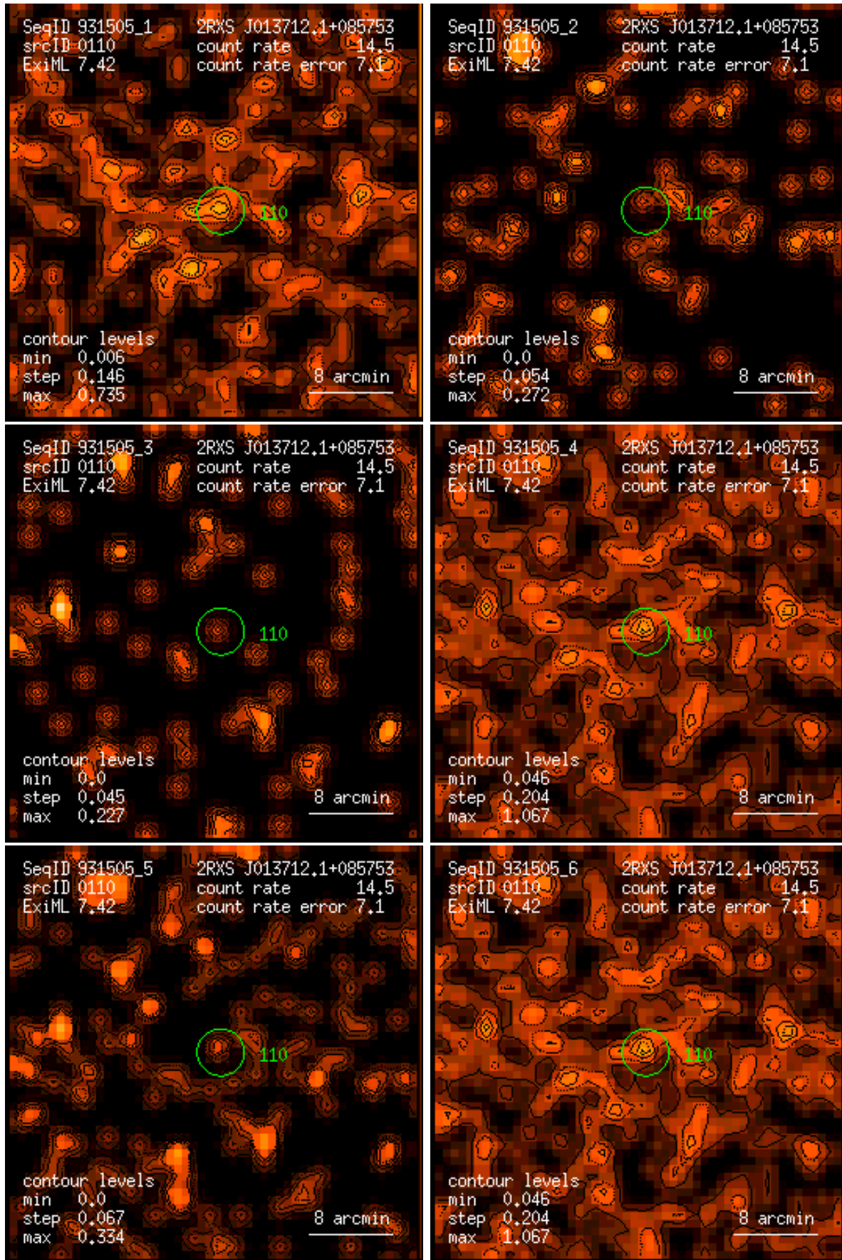
Figure 110: RASS 931505: detection 0110: band rate images, Gaussian filter: (1) PSPC channels 11 – 41, (2) 52 – 90, (3) 91 – 201, (4) 11 – 235, (5) 52 – 201, (6) 11 – 201. Broad band rates in counts/ks. Band rate contour levels in counts/ks/arcmin 2 .
