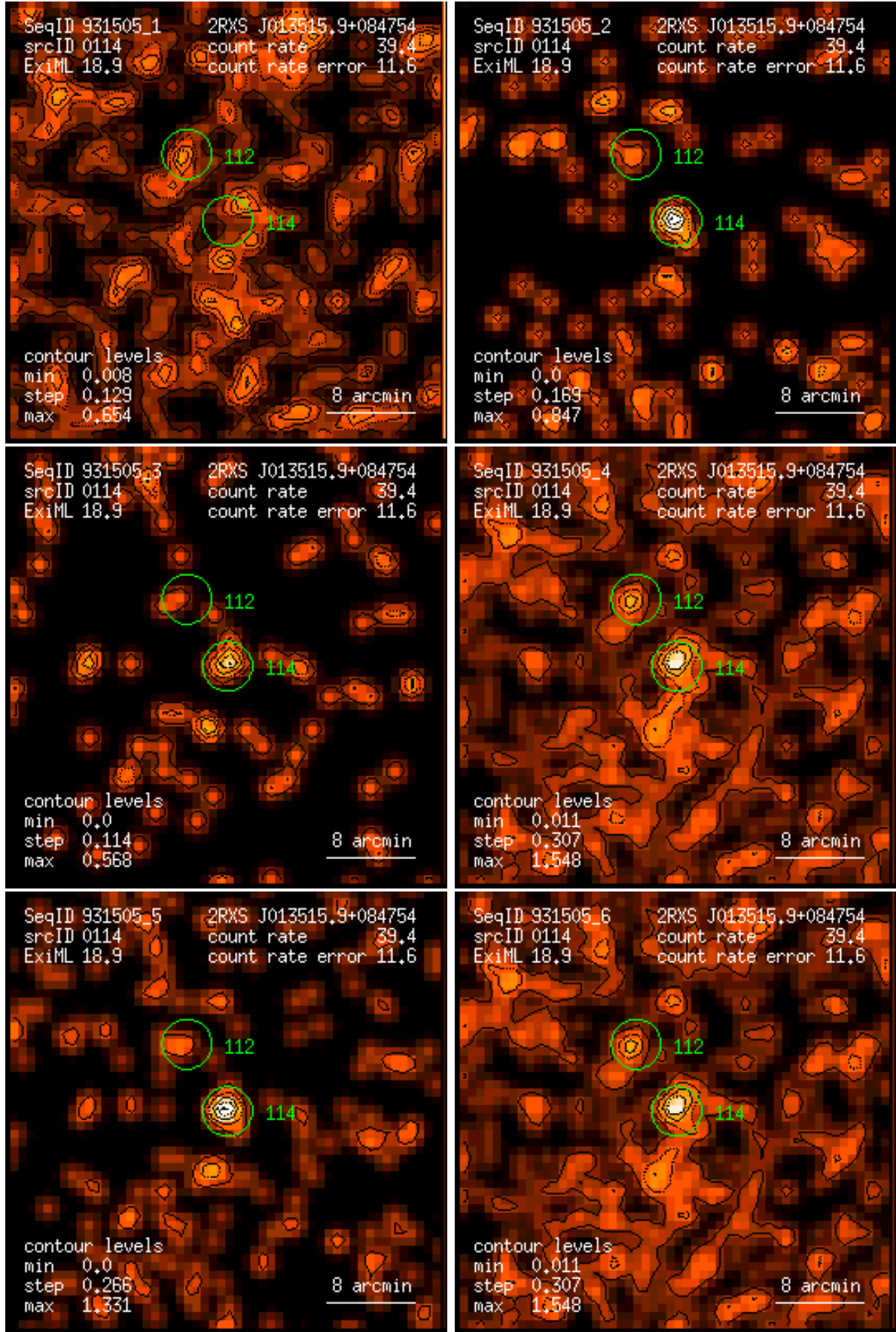
Figure 114: RASS 931505: detection 0114: band rate images, Gaussian filter: (1) PSPC channels 11 – 41, (2) 52 – 90, (3) 91 – 201, (4) 11 – 235, (5) 52 – 201, (6) 11 – 201. Broad band rates in counts/ks. Band rate contour levels in counts/ks/arcmin 2 .
