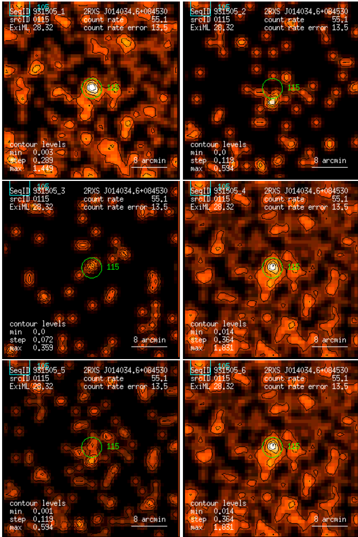
Figure 115: RASS 931505: detection 0115: band rate images, Gaussian filter: (1) PSPC channels 11 – 41, (2) 52 – 90, (3) 91 – 201, (4) 11 – 235, (5) 52 – 201, (6) 11 – 201. Broad band rates in counts/ks. Band rate contour levels in counts/ks/arcmin 2 .
