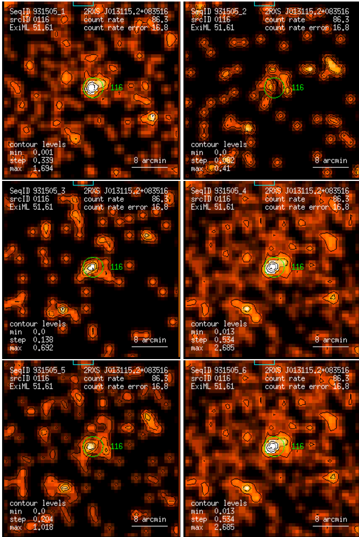
Figure 116: RASS 931505: detection 0116: band rate images, Gaussian filter: (1) PSPC channels 11 – 41, (2) 52 – 90, (3) 91 – 201, (4) 11 – 235, (5) 52 – 201, (6) 11 – 201. Broad band rates in counts/ks. Band rate contour levels in counts/ks/arcmin 2 .
