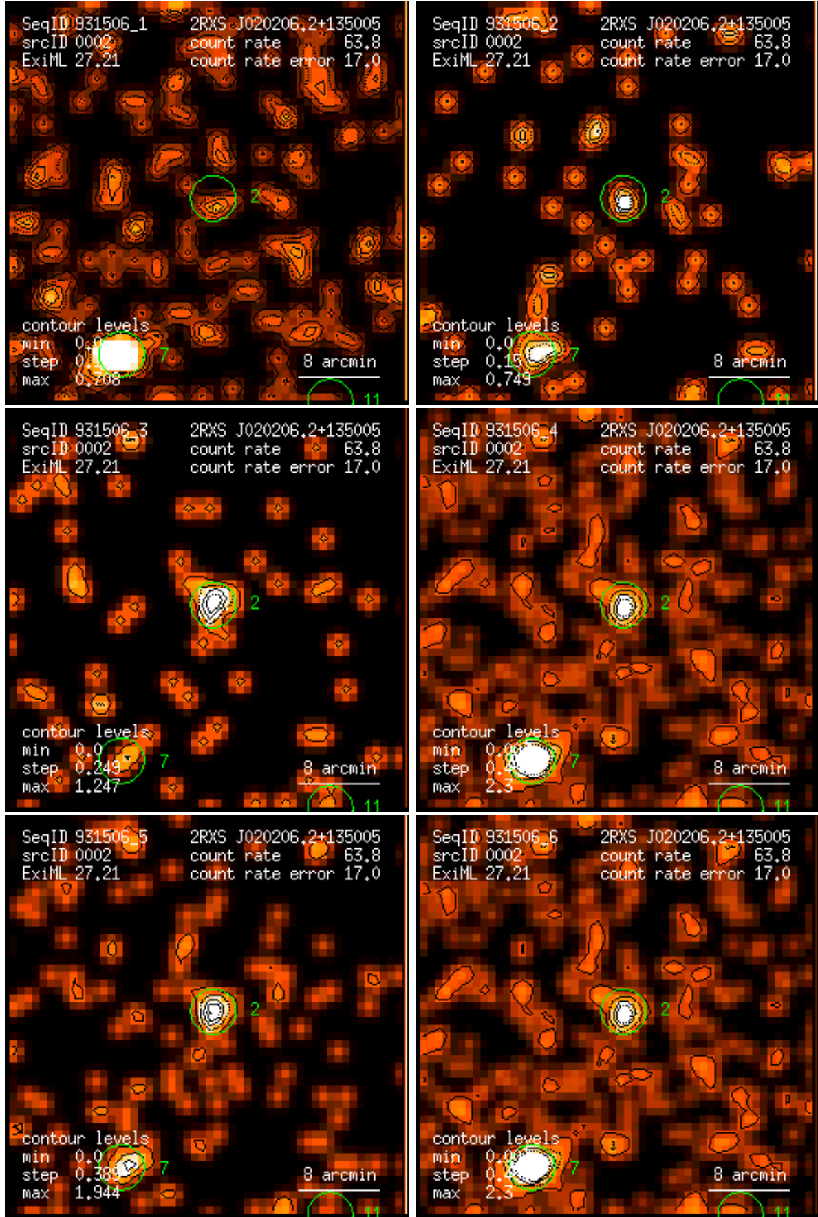
Figure 2: RASS 931506: detection 0002: band rate images, Gaussian filter: (1) PSPC channels 11 – 41, (2) 52 – 90, (3) 91 – 201, (4) 11 – 235, (5) 52 – 201, (6) 11 – 201. Broad band rates in counts/ks. Band rate contour levels in counts/ks/arcmin 2 .
