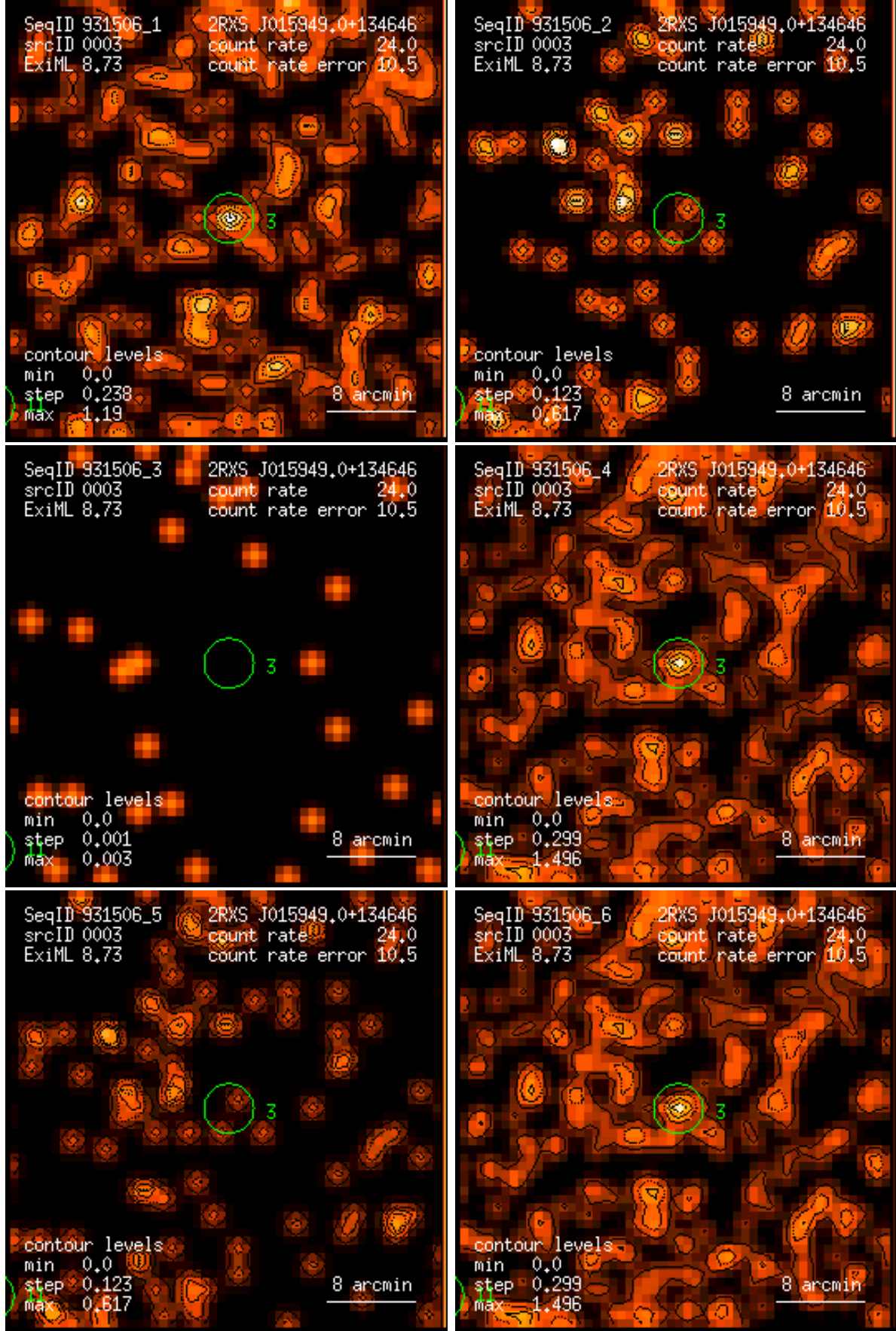
Figure 3: RASS 931506: detection 0003: band rate images, Gaussian filter: (1) PSPC channels 11 – 41, (2) 52 – 90, (3) 91 – 201, (4) 11 – 235, (5) 52 – 201, (6) 11 – 201. Broad band rates in counts/ks. Band rate contour levels in counts/ks/arcmin 2 .
