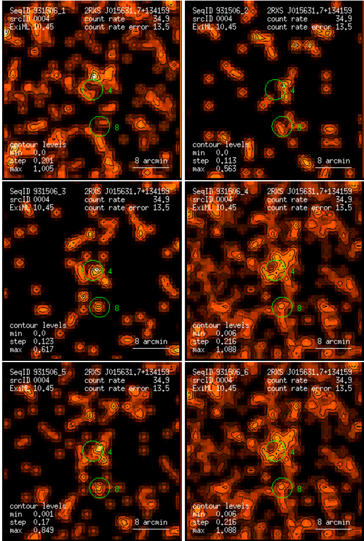
Figure 4: RASS 931506: detection 0004: band rate images, Gaussian filter: (1) PSPC channels 11 – 41, (2) 52 – 90, (3) 91 – 201, (4) 11 – 235, (5) 52 – 201, (6) 11 – 201. Broad band rates in counts/ks. Band rate contour levels in counts/ks/arcmin 2 .
