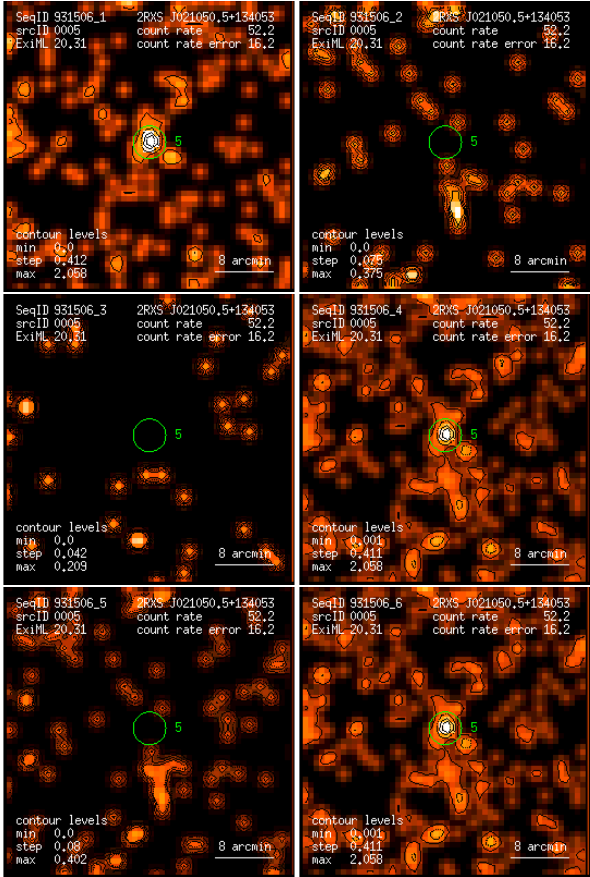
Figure 5: RASS 931506: detection 0005: band rate images, Gaussian filter: (1) PSPC channels 11 – 41, (2) 52 – 90, (3) 91 – 201, (4) 11 – 235, (5) 52 – 201, (6) 11 – 201. Broad band rates in counts/ks. Band rate contour levels in counts/ks/arcmin 2 .
