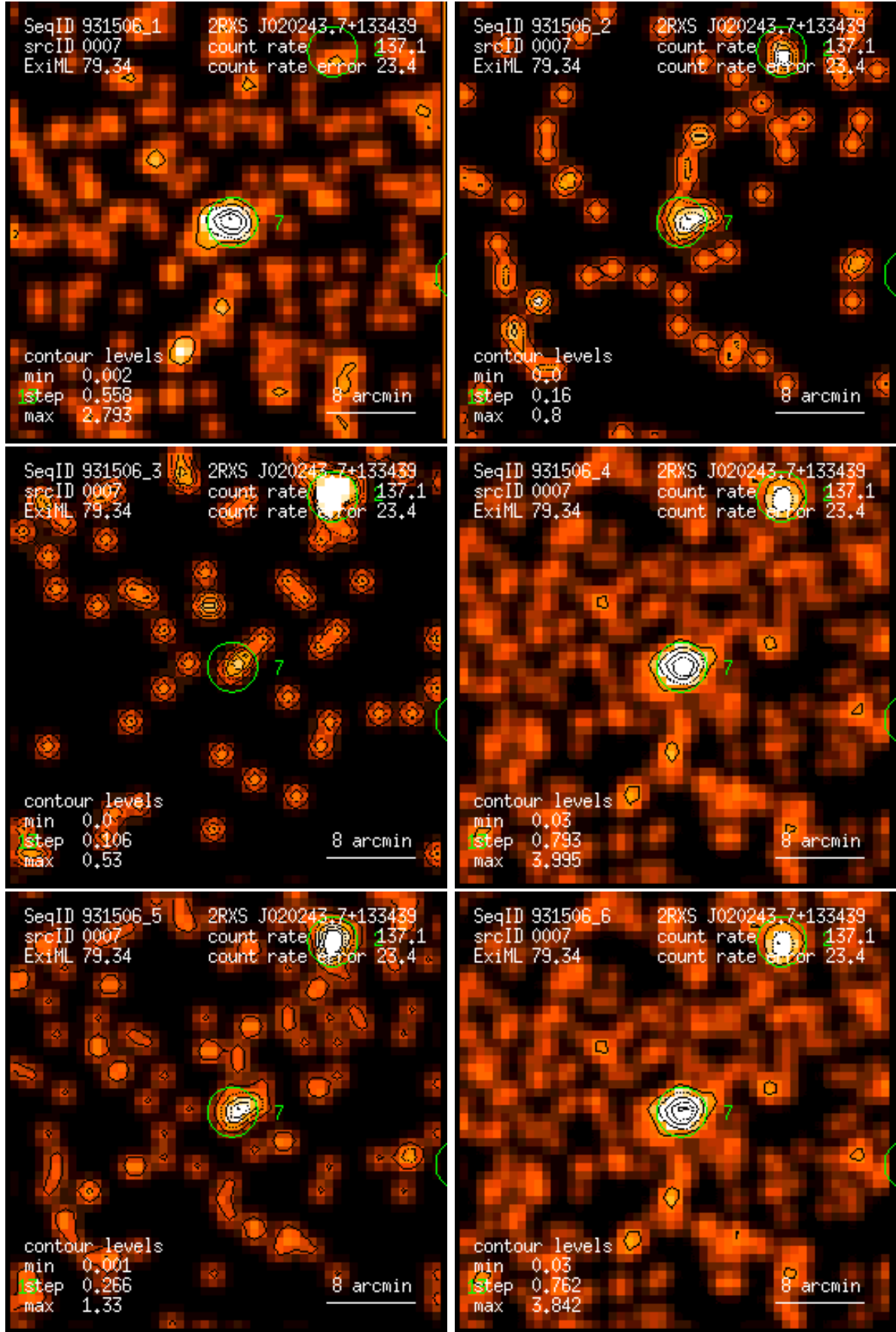
Figure 7: RASS 931506: detection 0007: band rate images, Gaussian filter: (1) PSPC channels 11 – 41, (2) 52 – 90, (3) 91 – 201, (4) 11 – 235, (5) 52 – 201, (6) 11 – 201. Broad band rates in counts/ks. Band rate contour levels in counts/ks/arcmin 2 .
