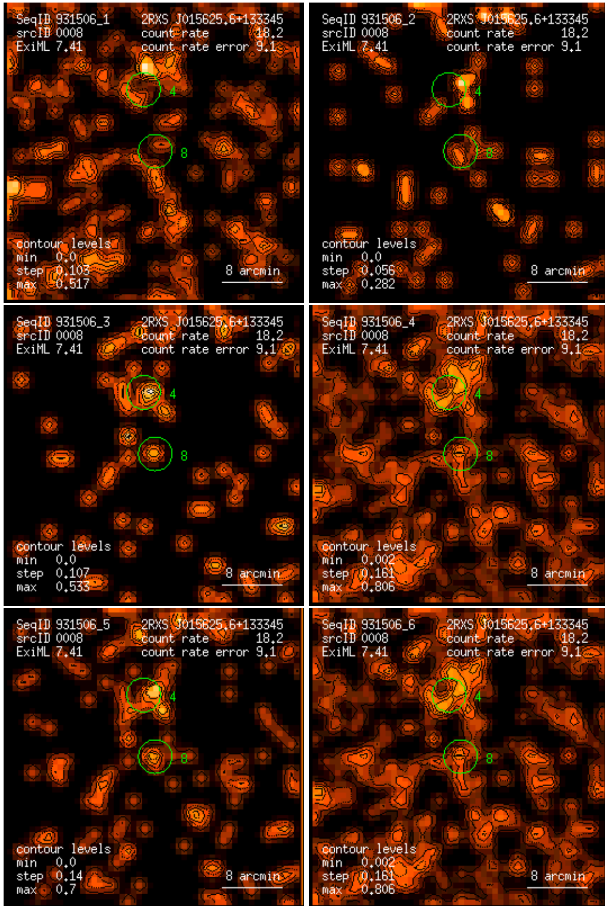
Figure 8: RASS 931506: detection 0008: band rate images, Gaussian filter: (1) PSPC channels 11 – 41, (2) 52 – 90, (3) 91 – 201, (4) 11 – 235, (5) 52 – 201, (6) 11 – 201. Broad band rates in counts/ks. Band rate contour levels in counts/ks/arcmin 2 .
