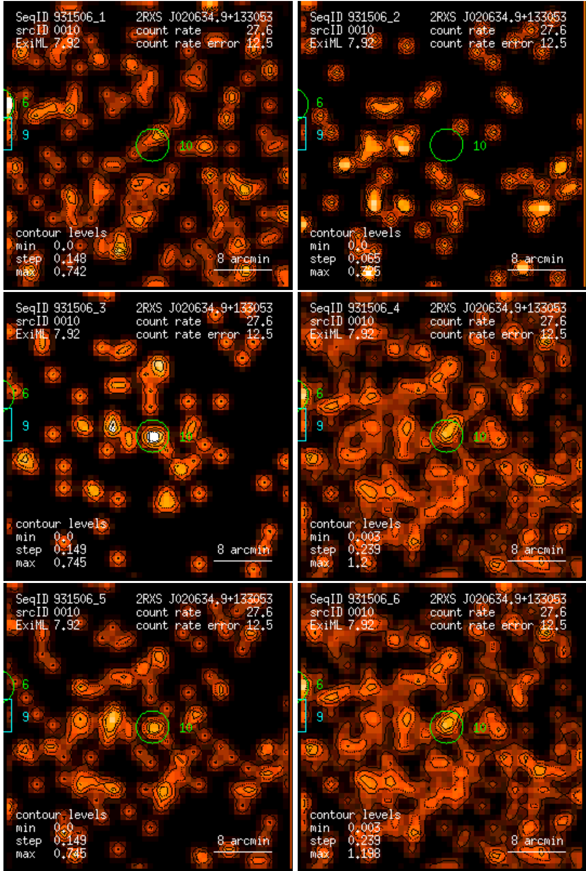
Figure 10: RASS 931506: detection 0010: band rate images, Gaussian filter: (1) PSPC channels 11 – 41, (2) 52 – 90, (3) 91 – 201, (4) 11 – 235, (5) 52 – 201, (6) 11 – 201. Broad band rates in counts/ks. Band rate contour levels in counts/ks/arcmin 2 .
