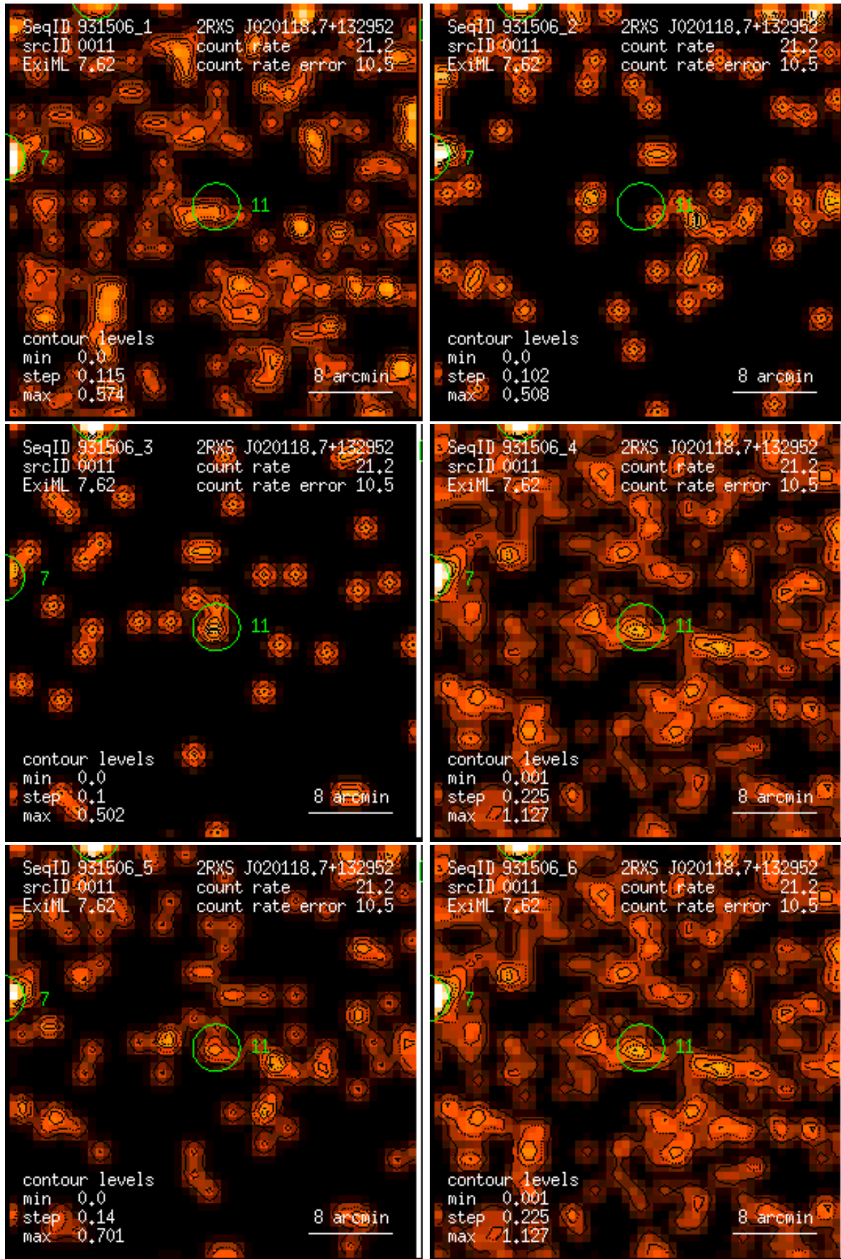
Figure 11: RASS 931506: detection 0011: band rate images, Gaussian filter: (1) PSPC channels 11 – 41, (2) 52 – 90, (3) 91 – 201, (4) 11 – 235, (5) 52 – 201, (6) 11 – 201. Broad band rates in counts/ks. Band rate contour levels in counts/ks/arcmin 2 .
