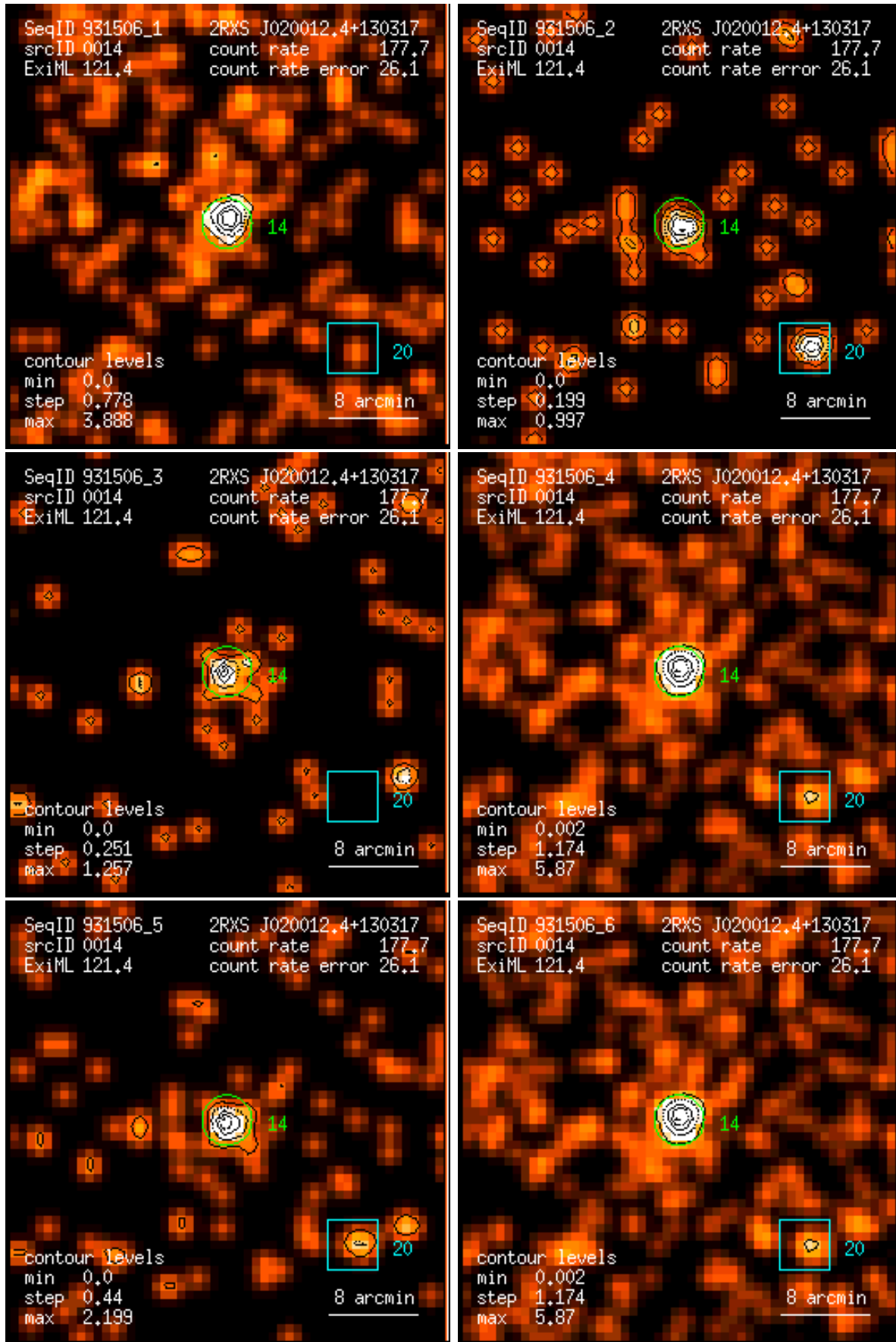
Figure 14: RASS 931506: detection 0014: band rate images, Gaussian filter: (1) PSPC channels 11 – 41, (2) 52 – 90, (3) 91 – 201, (4) 11 – 235, (5) 52 – 201, (6) 11 – 201. Broad band rates in counts/ks. Band rate contour levels in counts/ks/arcmin 2 .
