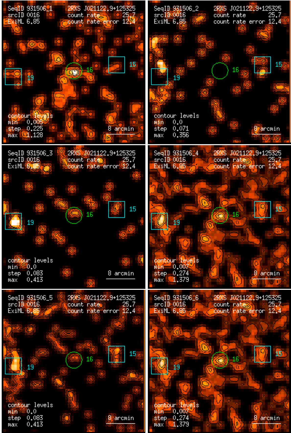
Figure 16: RASS 931506: detection 0016: band rate images, Gaussian filter: (1) PSPC channels 11 – 41, (2) 52 – 90, (3) 91 – 201, (4) 11 – 235, (5) 52 – 201, (6) 11 – 201. Broad band rates in counts/ks. Band rate contour levels in counts/ks/arcmin 2 .
