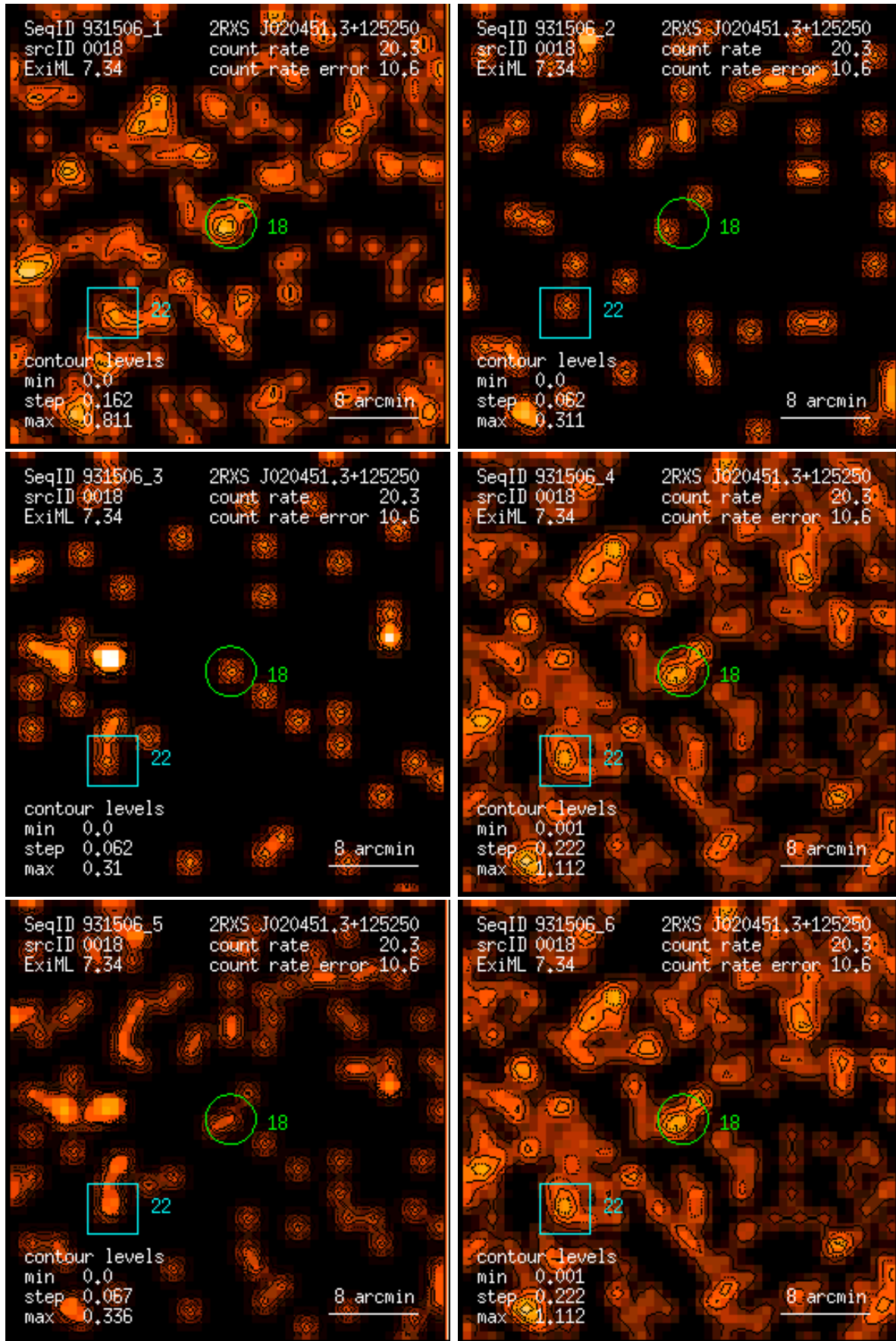
Figure 18: RASS 931506: detection 0018: band rate images, Gaussian filter: (1) PSPC channels 11 – 41, (2) 52 – 90, (3) 91 – 201, (4) 11 – 235, (5) 52 – 201, (6) 11 – 201. Broad band rates in counts/ks. Band rate contour levels in counts/ks/arcmin 2 .
