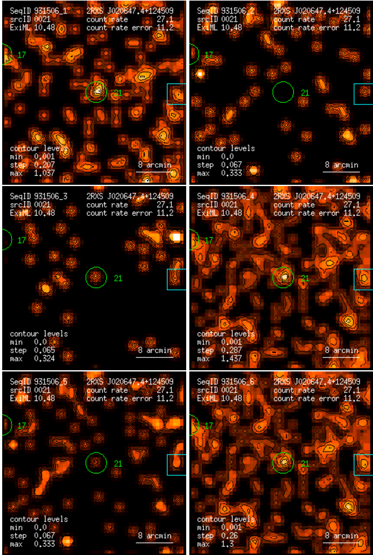
Figure 21: RASS 931506: detection 0021: band rate images, Gaussian filter: (1) PSPC channels 11 – 41, (2) 52 – 90, (3) 91 – 201, (4) 11 – 235, (5) 52 – 201, (6) 11 – 201. Broad band rates in counts/ks. Band rate contour levels in counts/ks/arcmin 2 .
