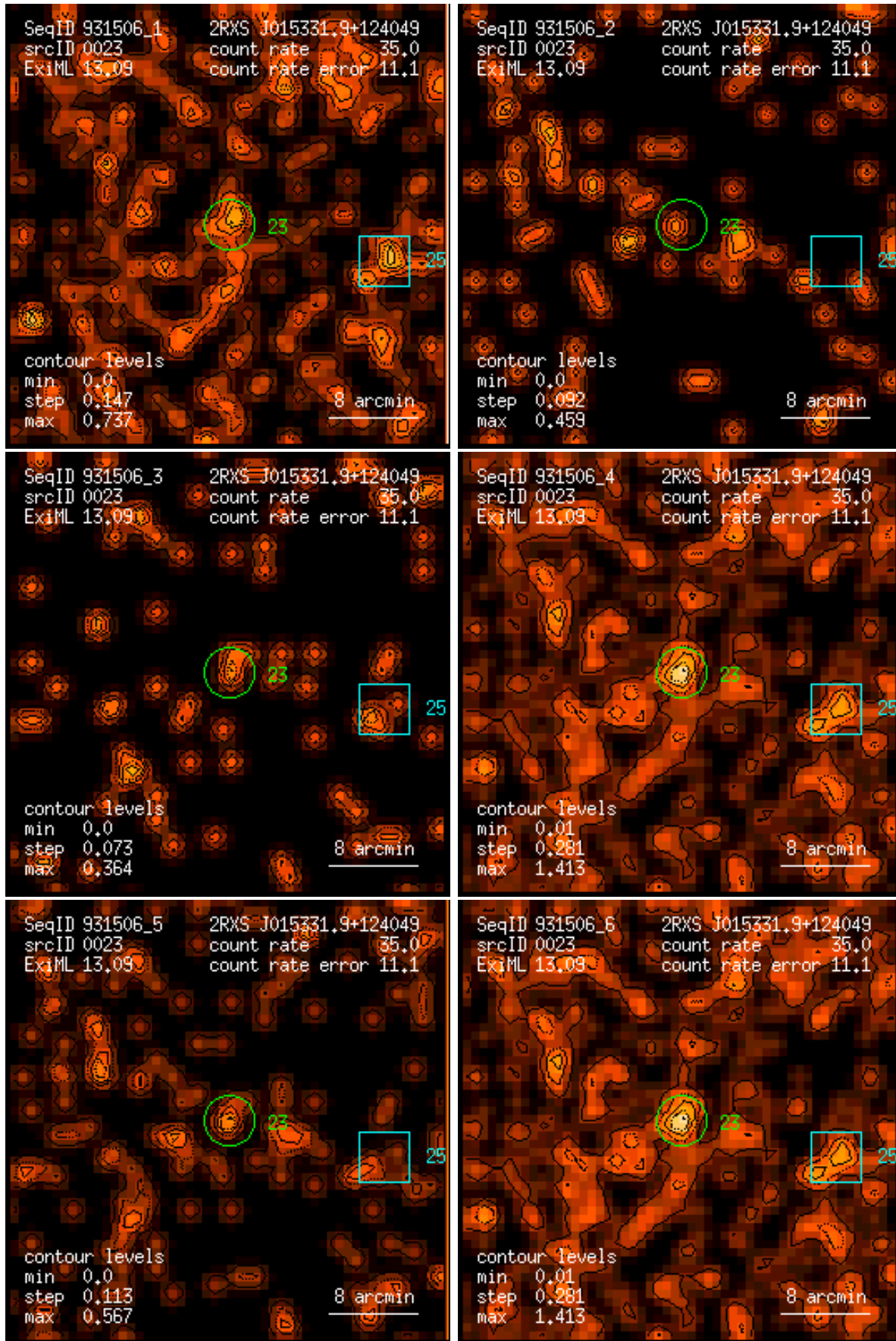
Figure 23: RASS 931506: detection 0023: band rate images, Gaussian filter: (1) PSPC channels 11 – 41, (2) 52 – 90, (3) 91 – 201, (4) 11 – 235, (5) 52 – 201, (6) 11 – 201. Broad band rates in counts/ks. Band rate contour levels in counts/ks/arcmin 2 .
