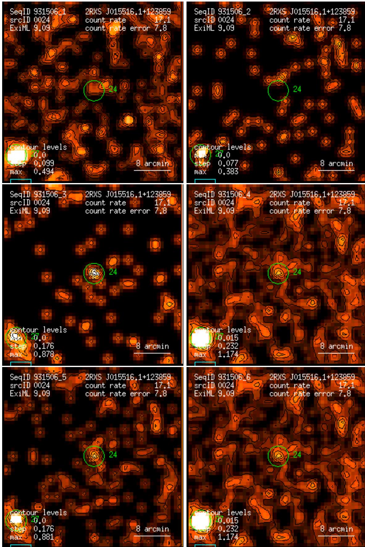
Figure 24: RASS 931506: detection 0024: band rate images, Gaussian filter: (1) PSPC channels 11 – 41, (2) 52 – 90, (3) 91 – 201, (4) 11 – 235, (5) 52 – 201, (6) 11 – 201. Broad band rates in counts/ks. Band rate contour levels in counts/ks/arcmin 2 .
