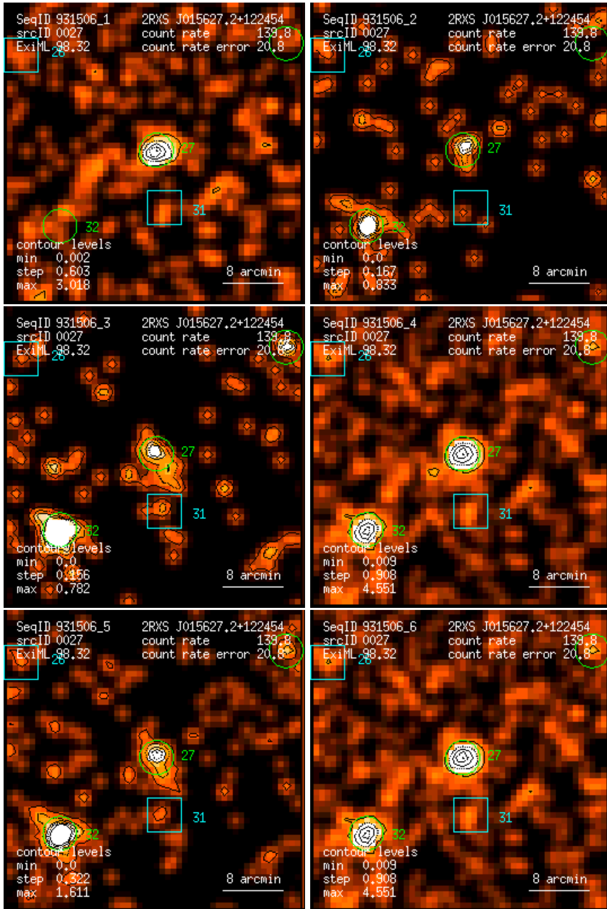
Figure 27: RASS 931506: detection 0027: band rate images, Gaussian filter: (1) PSPC channels 11 – 41, (2) 52 – 90, (3) 91 – 201, (4) 11 – 235, (5) 52 – 201, (6) 11 – 201. Broad band rates in counts/ks. Band rate contour levels in counts/ks/arcmin 2 .
