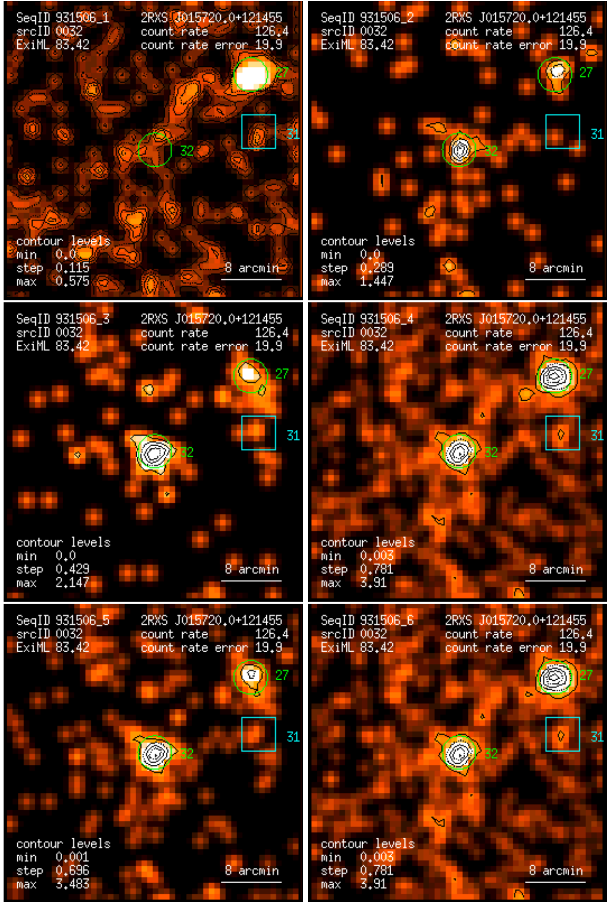
Figure 32: RASS 931506: detection 0032: band rate images, Gaussian filter: (1) PSPC channels 11 – 41, (2) 52 – 90, (3) 91 – 201, (4) 11 – 235, (5) 52 – 201, (6) 11 – 201. Broad band rates in counts/ks. Band rate contour levels in counts/ks/arcmin 2 .
