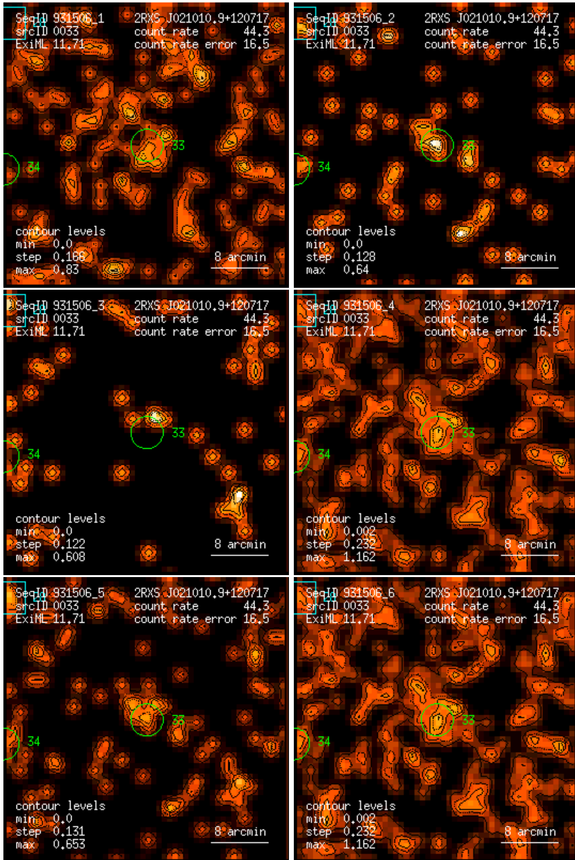
Figure 33: RASS 931506: detection 0033: band rate images, Gaussian filter: (1) PSPC channels 11 – 41, (2) 52 – 90, (3) 91 – 201, (4) 11 – 235, (5) 52 – 201, (6) 11 – 201. Broad band rates in counts/ks. Band rate contour levels in counts/ks/arcmin 2 .
