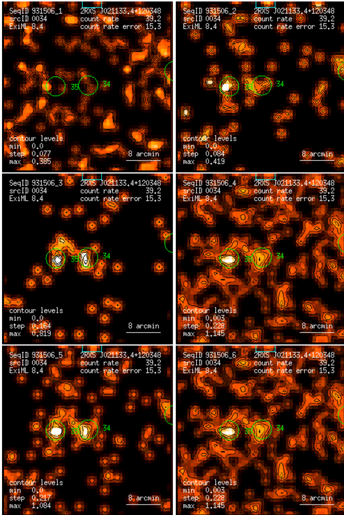
Figure 34: RASS 931506: detection 0034: band rate images, Gaussian filter: (1) PSPC channels 11 – 41, (2) 52 – 90, (3) 91 – 201, (4) 11 – 235, (5) 52 – 201, (6) 11 – 201. Broad band rates in counts/ks. Band rate contour levels in counts/ks/arcmin 2 .
