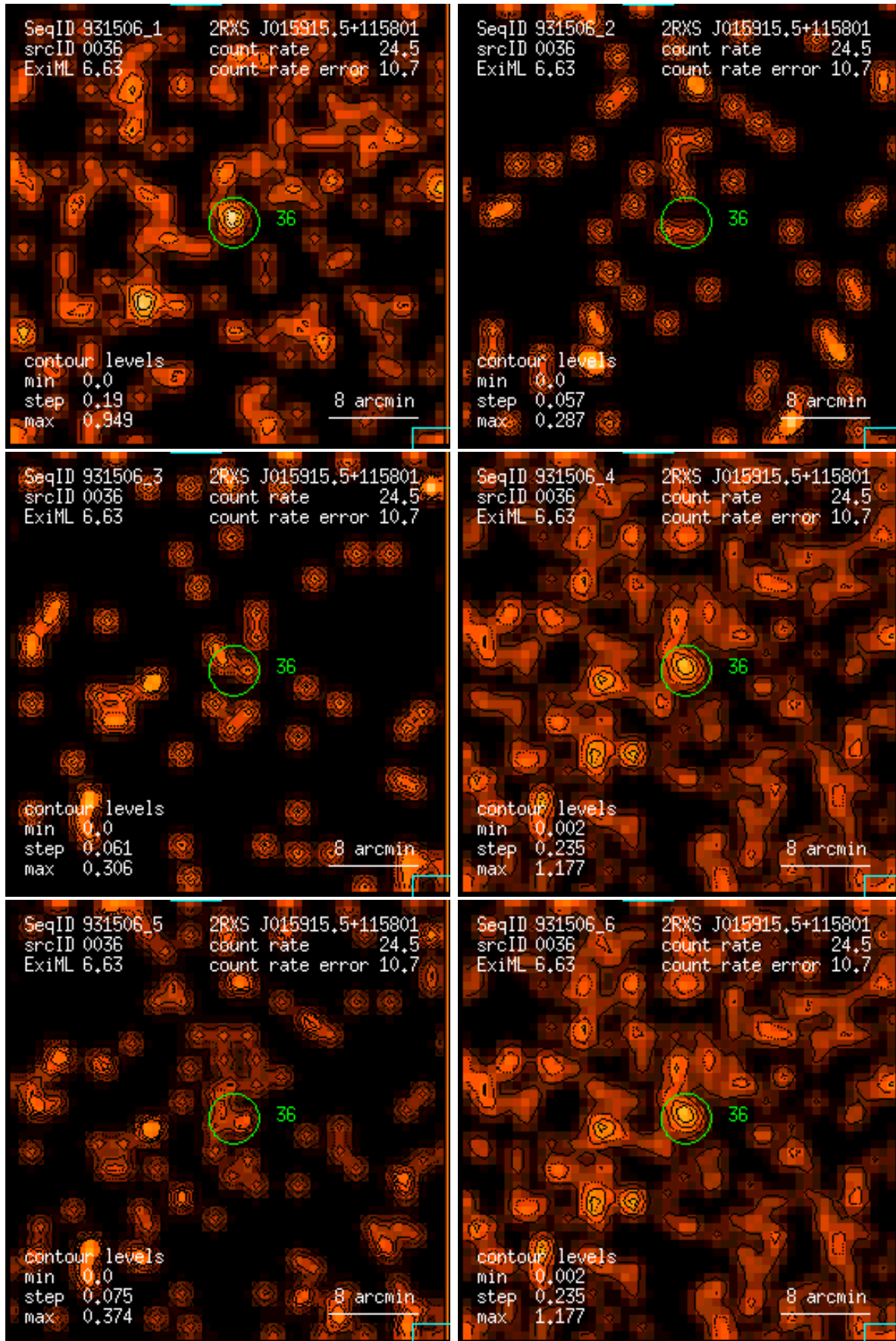
Figure 36: RASS 931506: detection 0036: band rate images, Gaussian filter: (1) PSPC channels 11 – 41, (2) 52 – 90, (3) 91 – 201, (4) 11 – 235, (5) 52 – 201, (6) 11 – 201. Broad band rates in counts/ks. Band rate contour levels in counts/ks/arcmin 2 .
