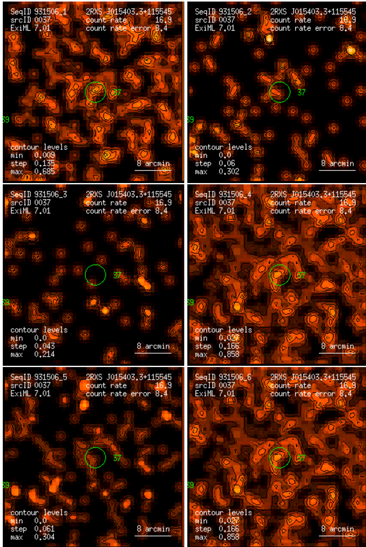
Figure 37: RASS 931506: detection 0037: band rate images, Gaussian filter: (1) PSPC channels 11 – 41, (2) 52 – 90, (3) 91 – 201, (4) 11 – 235, (5) 52 – 201, (6) 11 – 201. Broad band rates in counts/ks. Band rate contour levels in counts/ks/arcmin 2 .
