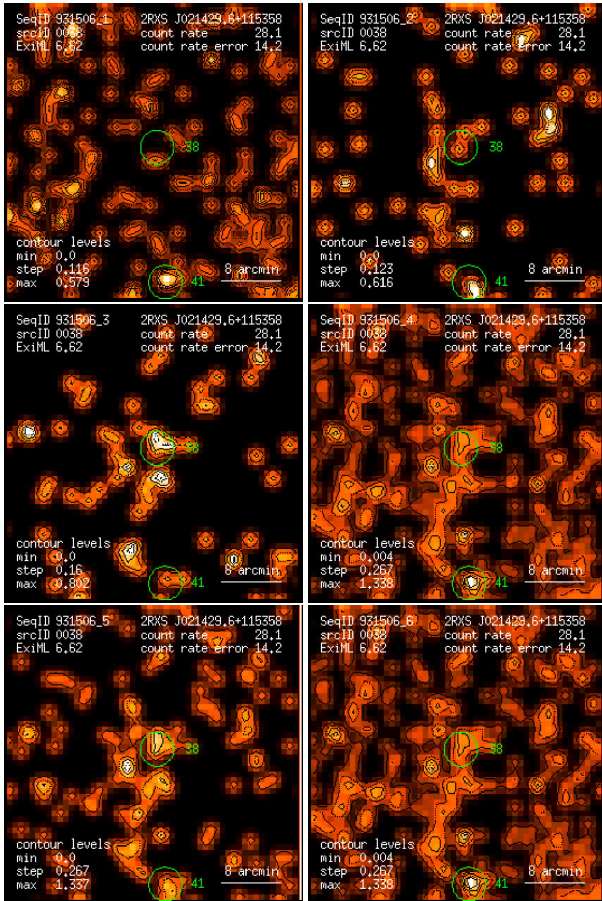
Figure 38: RASS 931506: detection 0038: band rate images, Gaussian filter: (1) PSPC channels 11 – 41, (2) 52 – 90, (3) 91 – 201, (4) 11 – 235, (5) 52 – 201, (6) 11 – 201. Broad band rates in counts/ks. Band rate contour levels in counts/ks/arcmin 2 .
