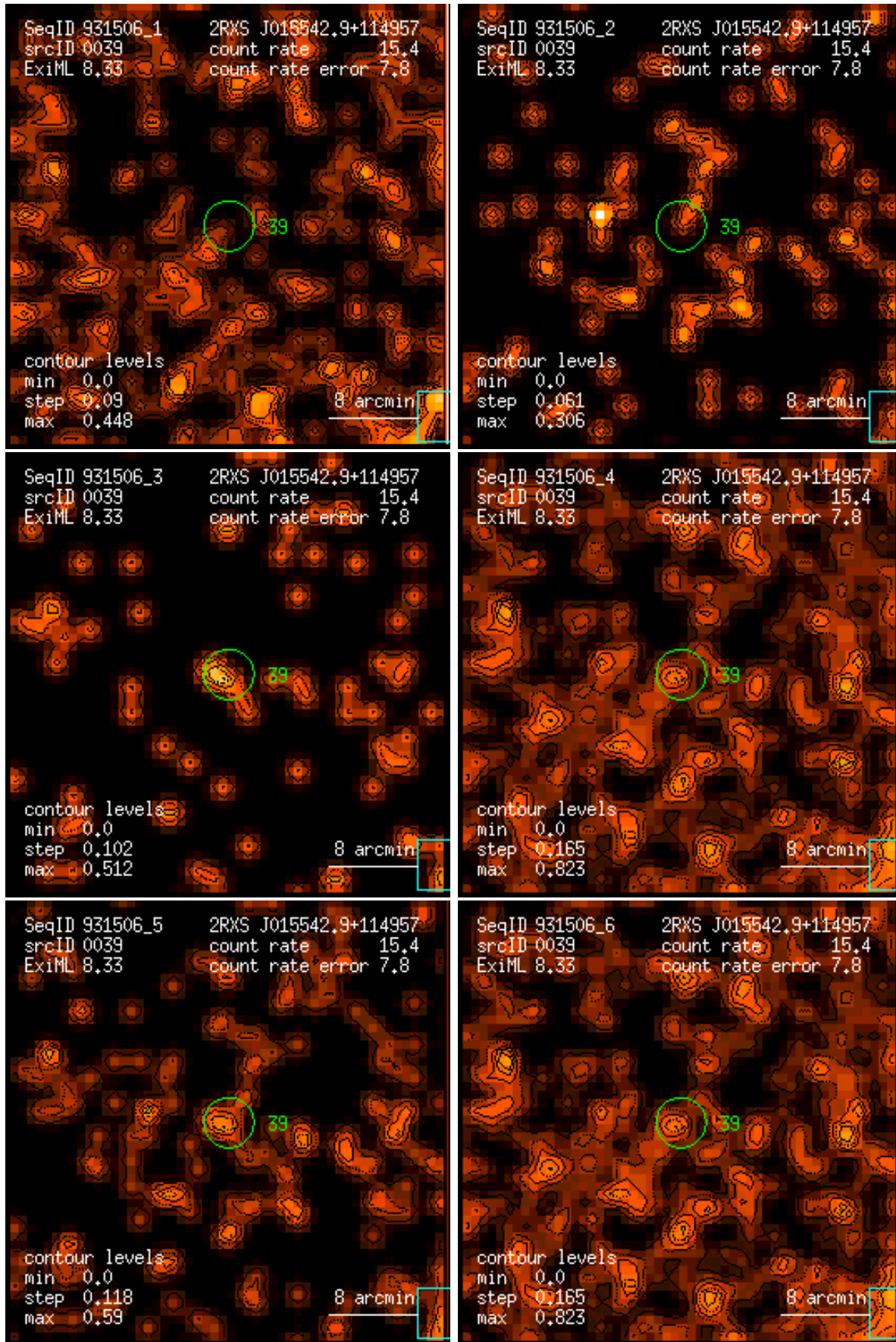
Figure 39: RASS 931506: detection 0039: band rate images, Gaussian filter: (1) PSPC channels 11 – 41, (2) 52 – 90, (3) 91 – 201, (4) 11 – 235, (5) 52 – 201, (6) 11 – 201. Broad band rates in counts/ks. Band rate contour levels in counts/ks/arcmin 2 .
