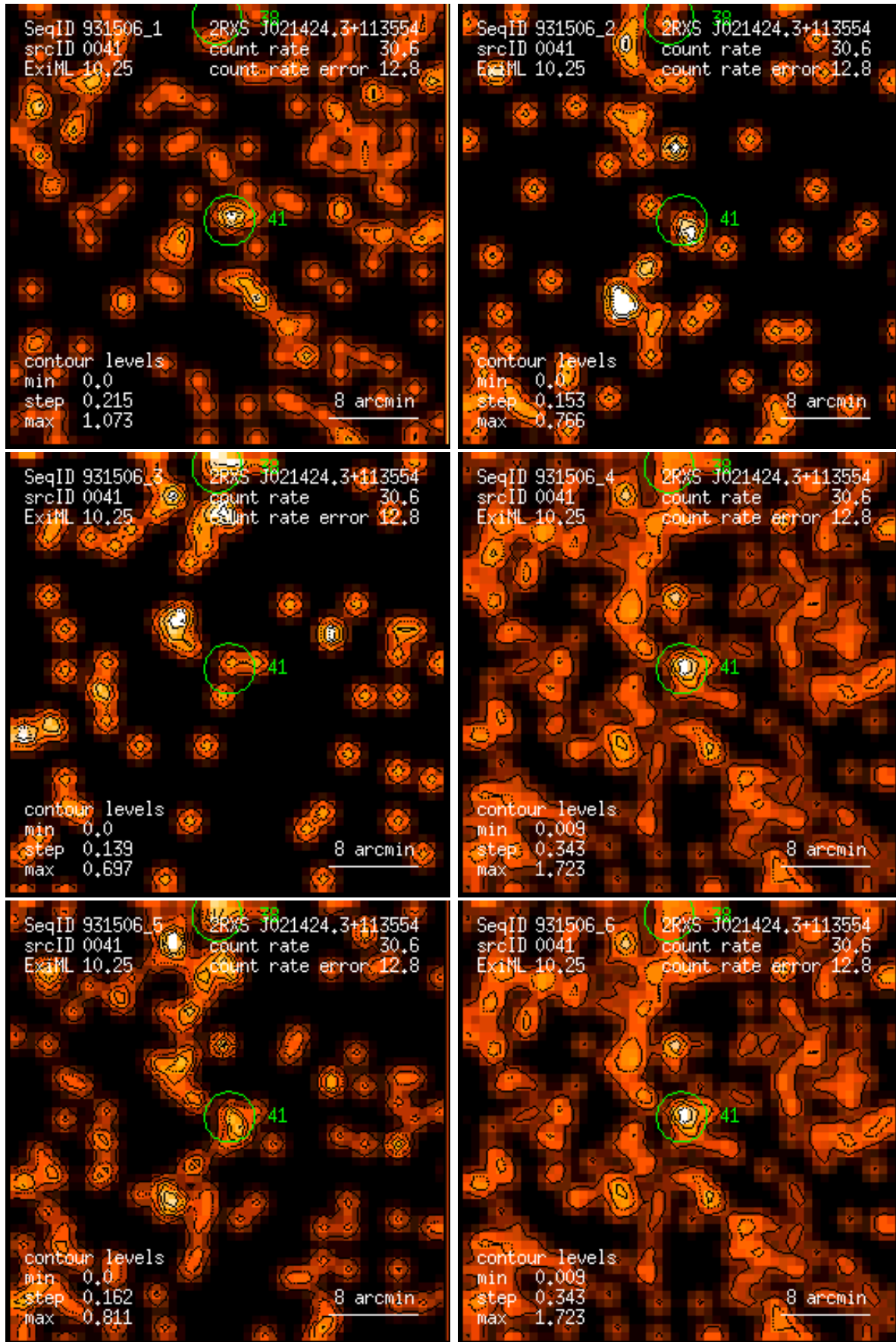
Figure 41: RASS 931506: detection 0041: band rate images, Gaussian filter: (1) PSPC channels 11 – 41, (2) 52 – 90, (3) 91 – 201, (4) 11 – 235, (5) 52 – 201, (6) 11 – 201. Broad band rates in counts/ks. Band rate contour levels in counts/ks/arcmin 2 .
