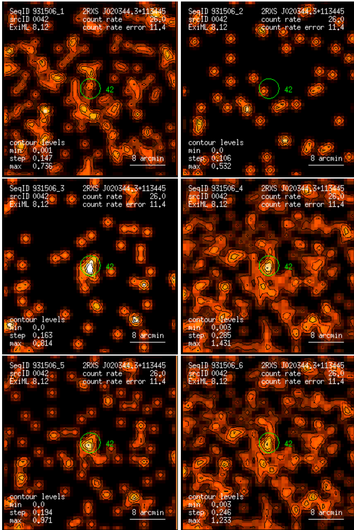
Figure 42: RASS 931506: detection 0042: band rate images, Gaussian filter: (1) PSPC channels 11 – 41, (2) 52 – 90, (3) 91 – 201, (4) 11 – 235, (5) 52 – 201, (6) 11 – 201. Broad band rates in counts/ks. Band rate contour levels in counts/ks/arcmin 2 .
