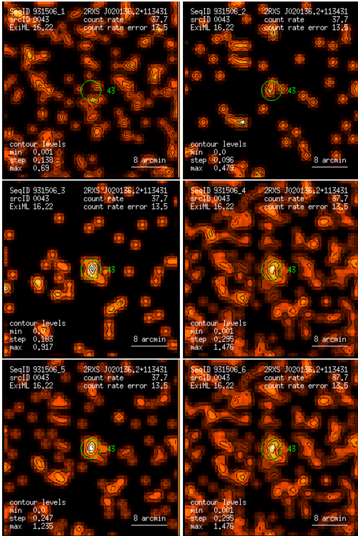
Figure 43: RASS 931506: detection 0043: band rate images, Gaussian filter: (1) PSPC channels 11 – 41, (2) 52 – 90, (3) 91 – 201, (4) 11 – 235, (5) 52 – 201, (6) 11 – 201. Broad band rates in counts/ks. Band rate contour levels in counts/ks/arcmin 2 .
