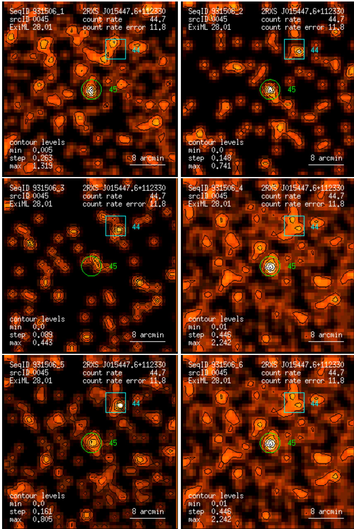
Figure 45: RASS 931506: detection 0045: band rate images, Gaussian filter: (1) PSPC channels 11 – 41, (2) 52 – 90, (3) 91 – 201, (4) 11 – 235, (5) 52 – 201, (6) 11 – 201. Broad band rates in counts/ks. Band rate contour levels in counts/ks/arcmin 2 .
