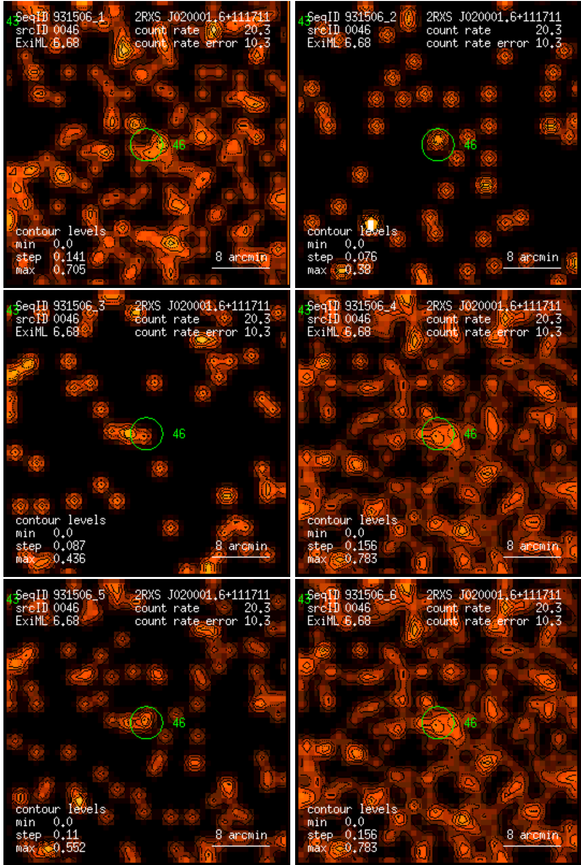
Figure 46: RASS 931506: detection 0046: band rate images, Gaussian filter: (1) PSPC channels 11 – 41, (2) 52 – 90, (3) 91 – 201, (4) 11 – 235, (5) 52 – 201, (6) 11 – 201. Broad band rates in counts/ks. Band rate contour levels in counts/ks/arcmin 2 .
