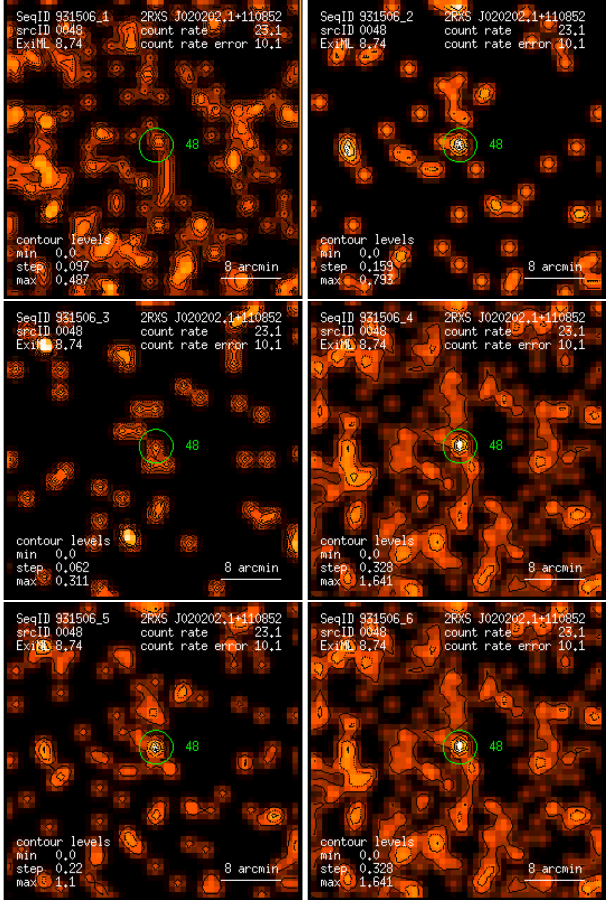
Figure 48: RASS 931506: detection 0048: band rate images, Gaussian filter: (1) PSPC channels 11 – 41, (2) 52 – 90, (3) 91 – 201, (4) 11 – 235, (5) 52 – 201, (6) 11 – 201. Broad band rates in counts/ks. Band rate contour levels in counts/ks/arcmin 2 .
