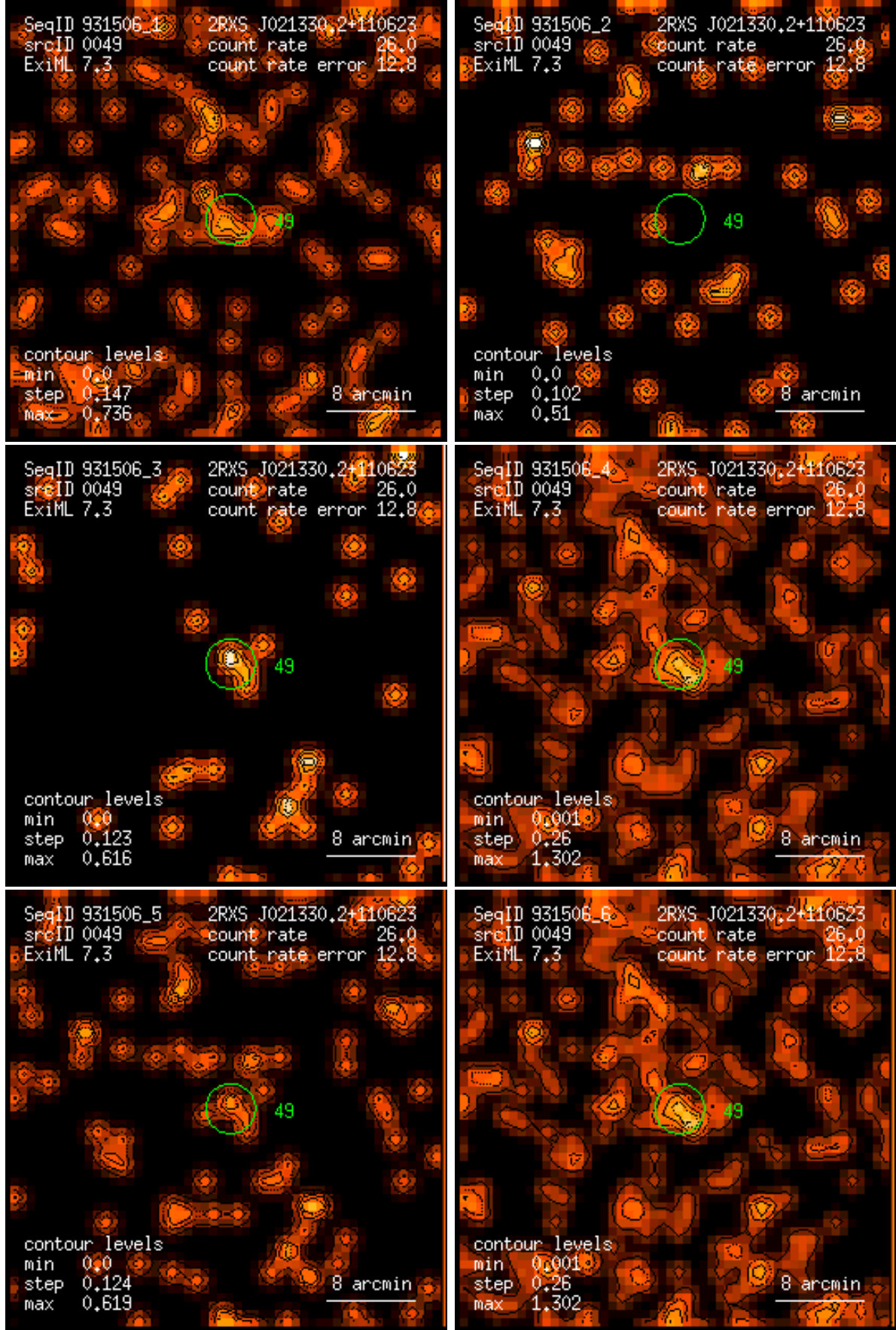
Figure 49: RASS 931506: detection 0049: band rate images, Gaussian filter: (1) PSPC channels 11 – 41, (2) 52 – 90, (3) 91 – 201, (4) 11 – 235, (5) 52 – 201, (6) 11 – 201. Broad band rates in counts/ks. Band rate contour levels in counts/ks/arcmin 2 .
