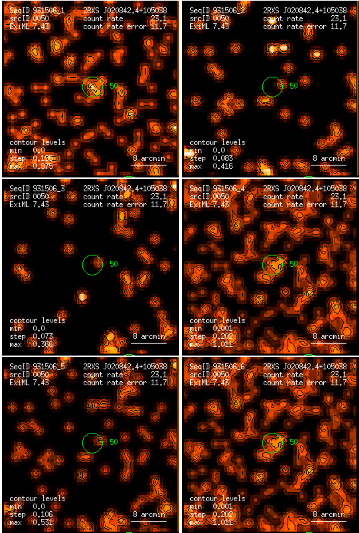
Figure 50: RASS 931506: detection 0050: band rate images, Gaussian filter: (1) PSPC channels 11 – 41, (2) 52 – 90, (3) 91 – 201, (4) 11 – 235, (5) 52 – 201, (6) 11 – 201. Broad band rates in counts/ks. Band rate contour levels in counts/ks/arcmin 2 .
