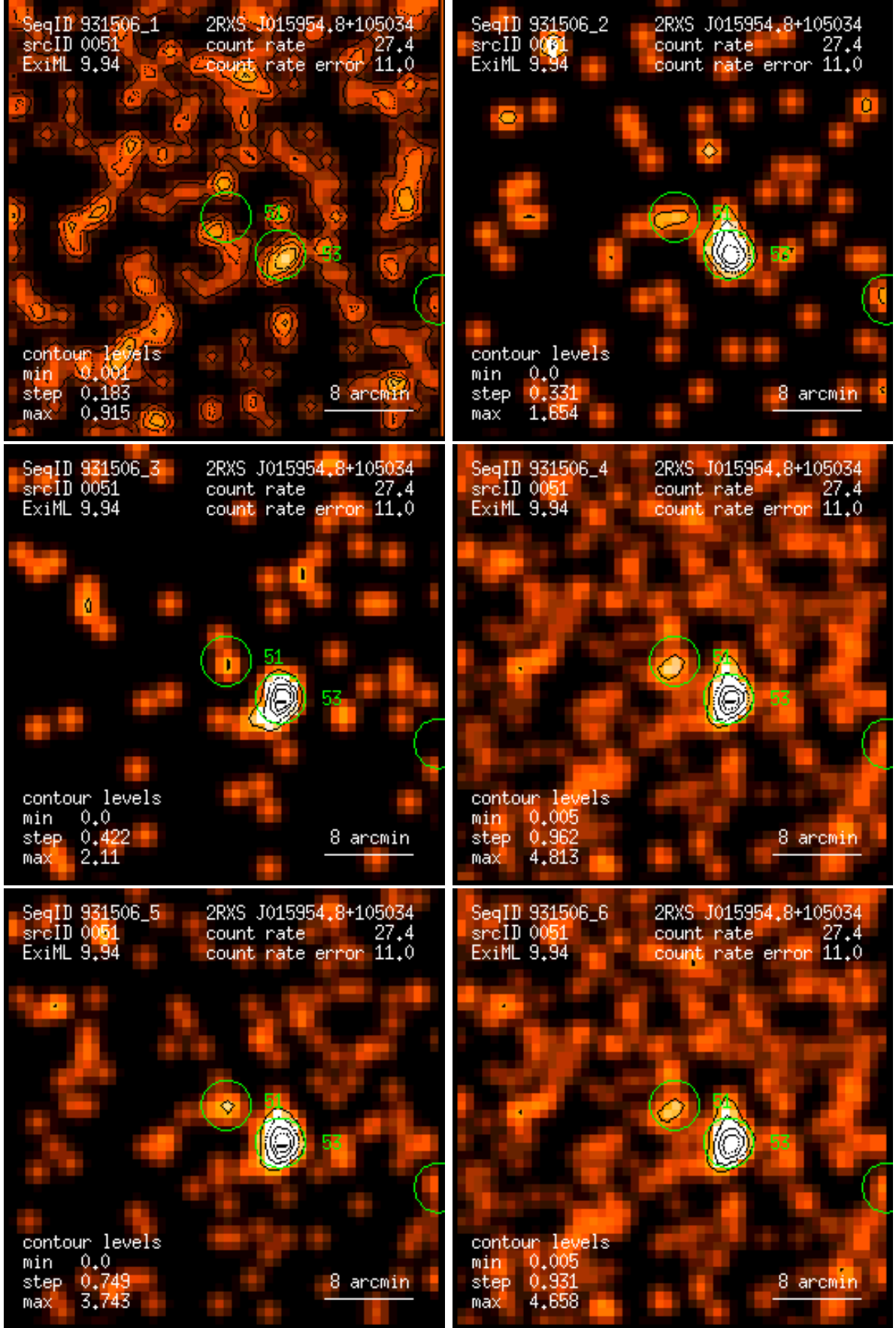
Figure 51: RASS 931506: detection 0051: band rate images, Gaussian filter: (1) PSPC channels 11 – 41, (2) 52 – 90, (3) 91 – 201, (4) 11 – 235, (5) 52 – 201, (6) 11 – 201. Broad band rates in counts/ks. Band rate contour levels in counts/ks/arcmin 2 .
