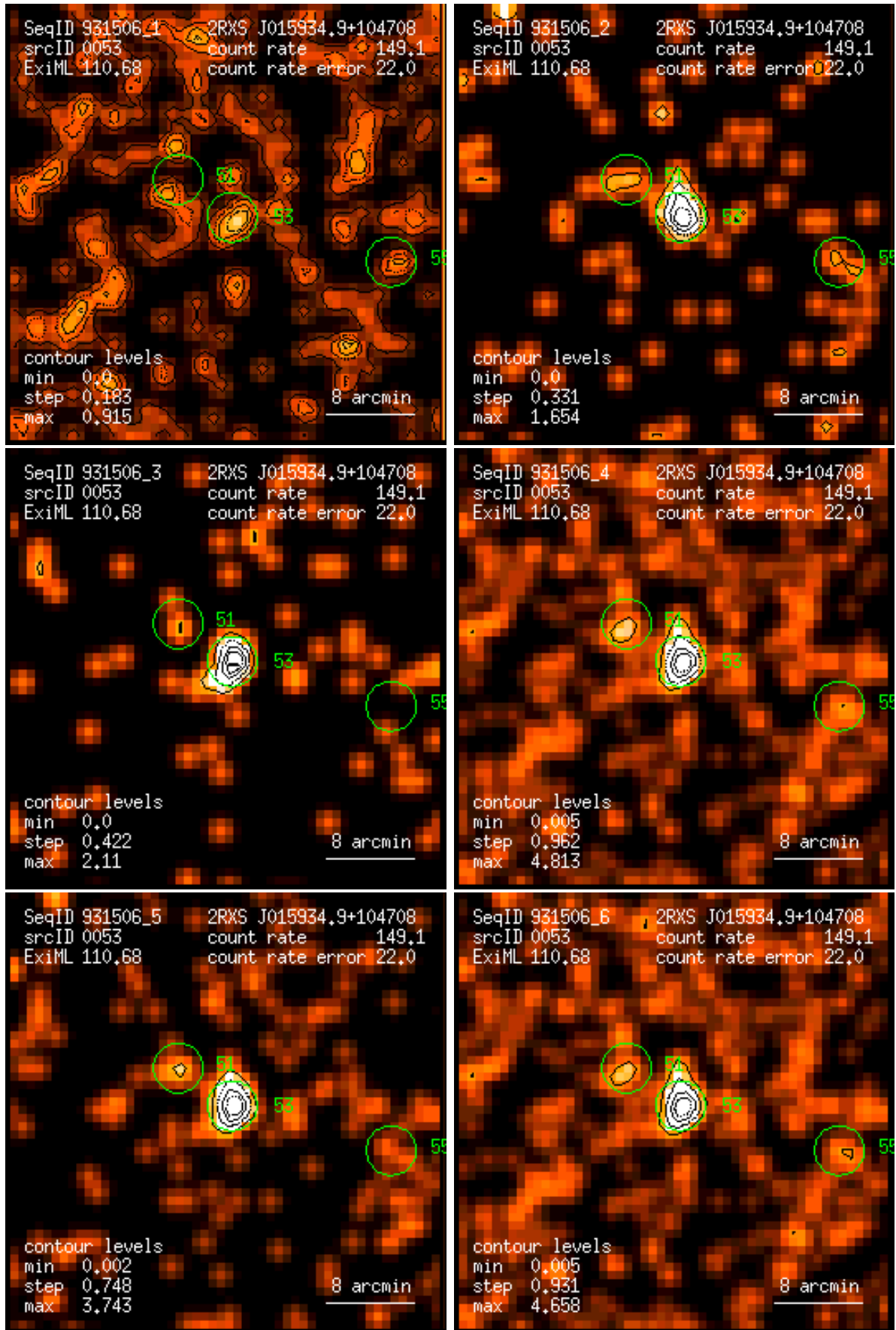
Figure 53: RASS 931506: detection 0053: band rate images, Gaussian filter: (1) PSPC channels 11 – 41, (2) 52 – 90, (3) 91 – 201, (4) 11 – 235, (5) 52 – 201, (6) 11 – 201. Broad band rates in counts/ks. Band rate contour levels in counts/ks/arcmin 2 .
