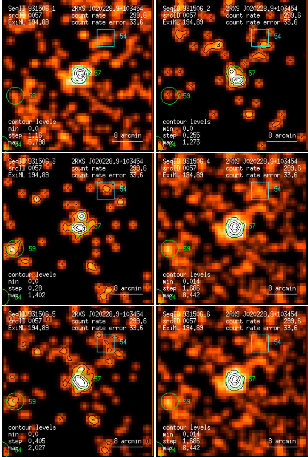
Figure 57: RASS 931506: detection 0057: band rate images, Gaussian filter: (1) PSPC channels 11 – 41, (2) 52 – 90, (3) 91 – 201, (4) 11 – 235, (5) 52 – 201, (6) 11 – 201. Broad band rates in counts/ks. Band rate contour levels in counts/ks/arcmin 2 .
