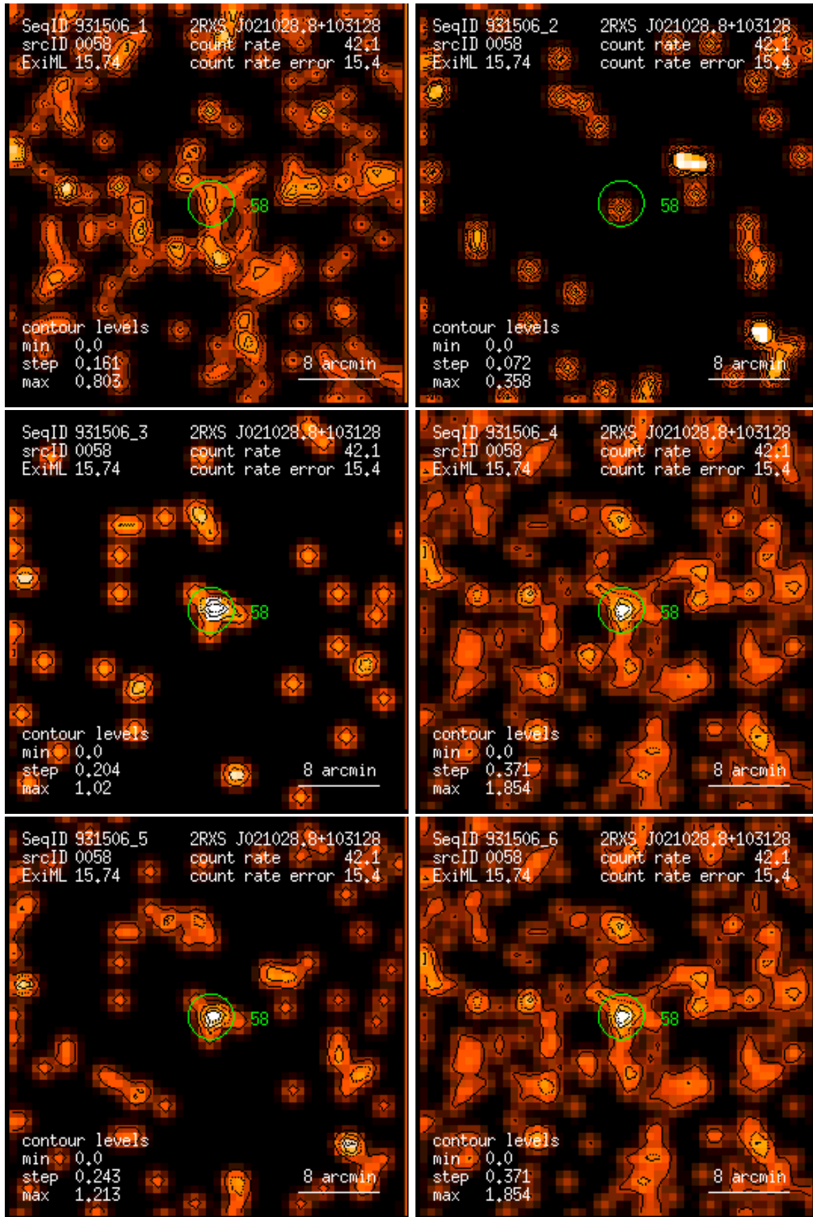
Figure 58: RASS 931506: detection 0058: band rate images, Gaussian filter: (1) PSPC channels 11 – 41, (2) 52 – 90, (3) 91 – 201, (4) 11 – 235, (5) 52 – 201, (6) 11 – 201. Broad band rates in counts/ks. Band rate contour levels in counts/ks/arcmin 2 .
