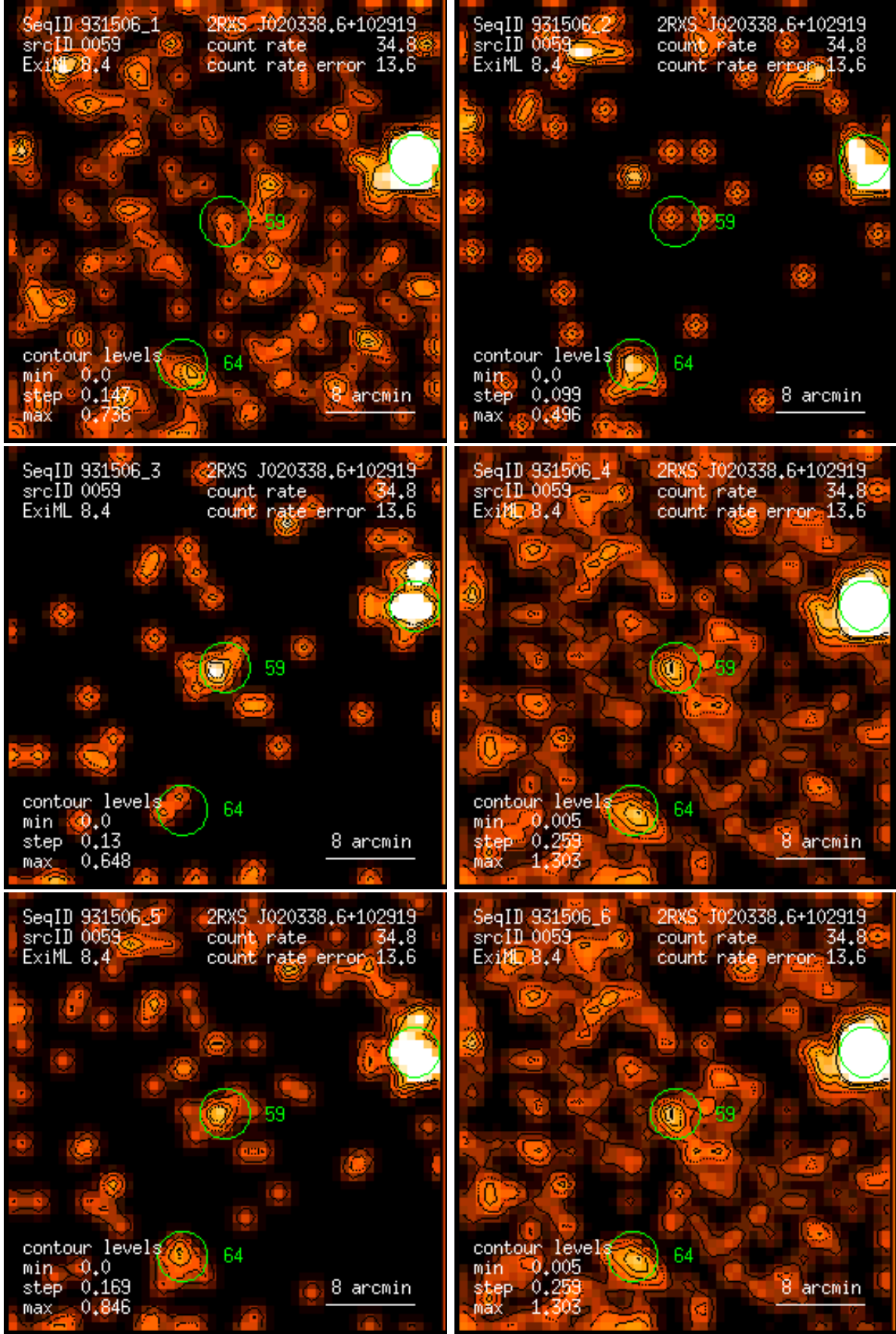
Figure 59: RASS 931506: detection 0059: band rate images, Gaussian filter: (1) PSPC channels 11 – 41, (2) 52 – 90, (3) 91 – 201, (4) 11 – 235, (5) 52 – 201, (6) 11 – 201. Broad band rates in counts/ks. Band rate contour levels in counts/ks/arcmin 2 .
