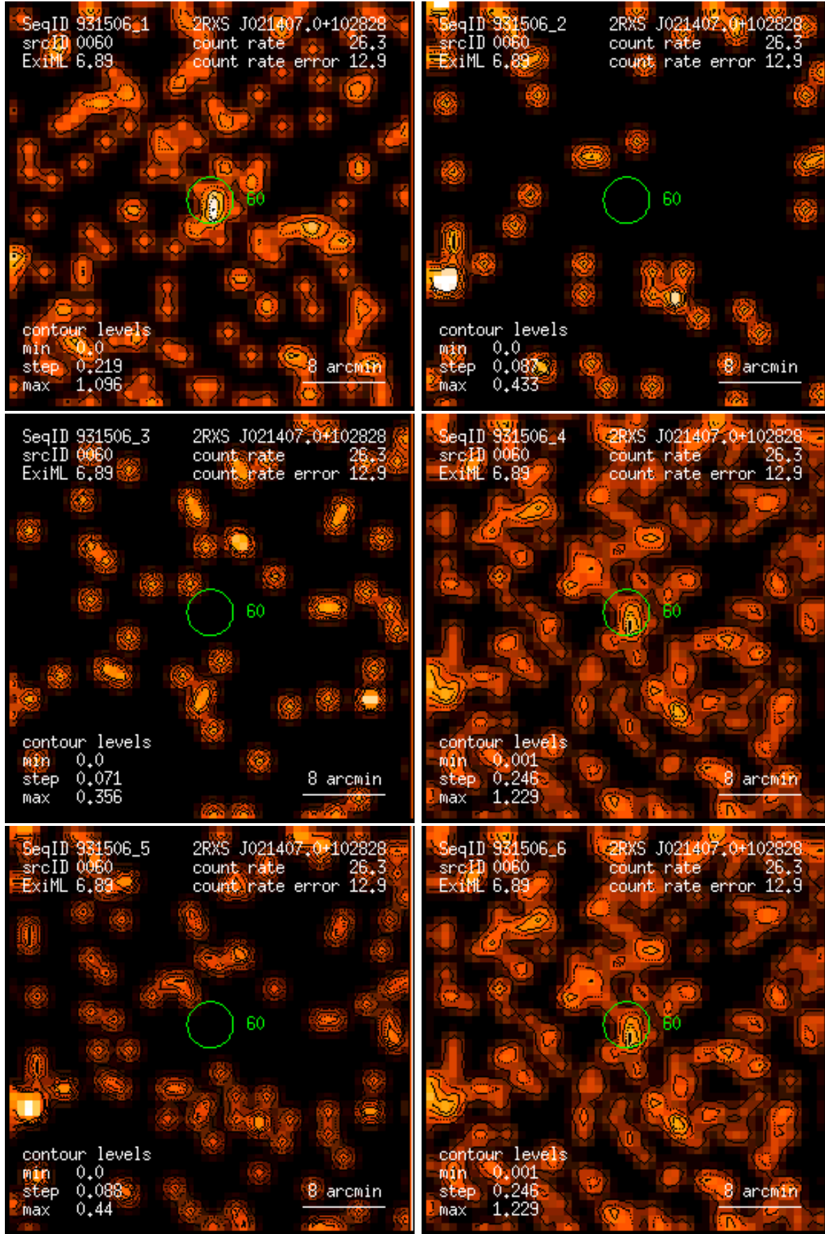
Figure 60: RASS 931506: detection 0060: band rate images, Gaussian filter: (1) PSPC channels 11 – 41, (2) 52 – 90, (3) 91 – 201, (4) 11 – 235, (5) 52 – 201, (6) 11 – 201. Broad band rates in counts/ks. Band rate contour levels in counts/ks/arcmin 2 .
