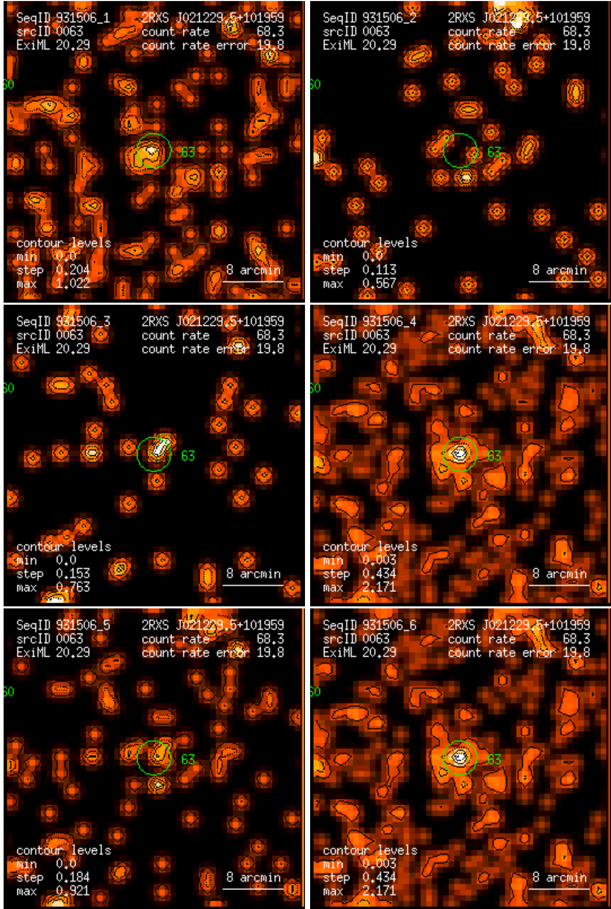
Figure 63: RASS 931506: detection 0063: band rate images, Gaussian filter: (1) PSPC channels 11 – 41, (2) 52 – 90, (3) 91 – 201, (4) 11 – 235, (5) 52 – 201, (6) 11 – 201. Broad band rates in counts/ks. Band rate contour levels in counts/ks/arcmin 2 .
