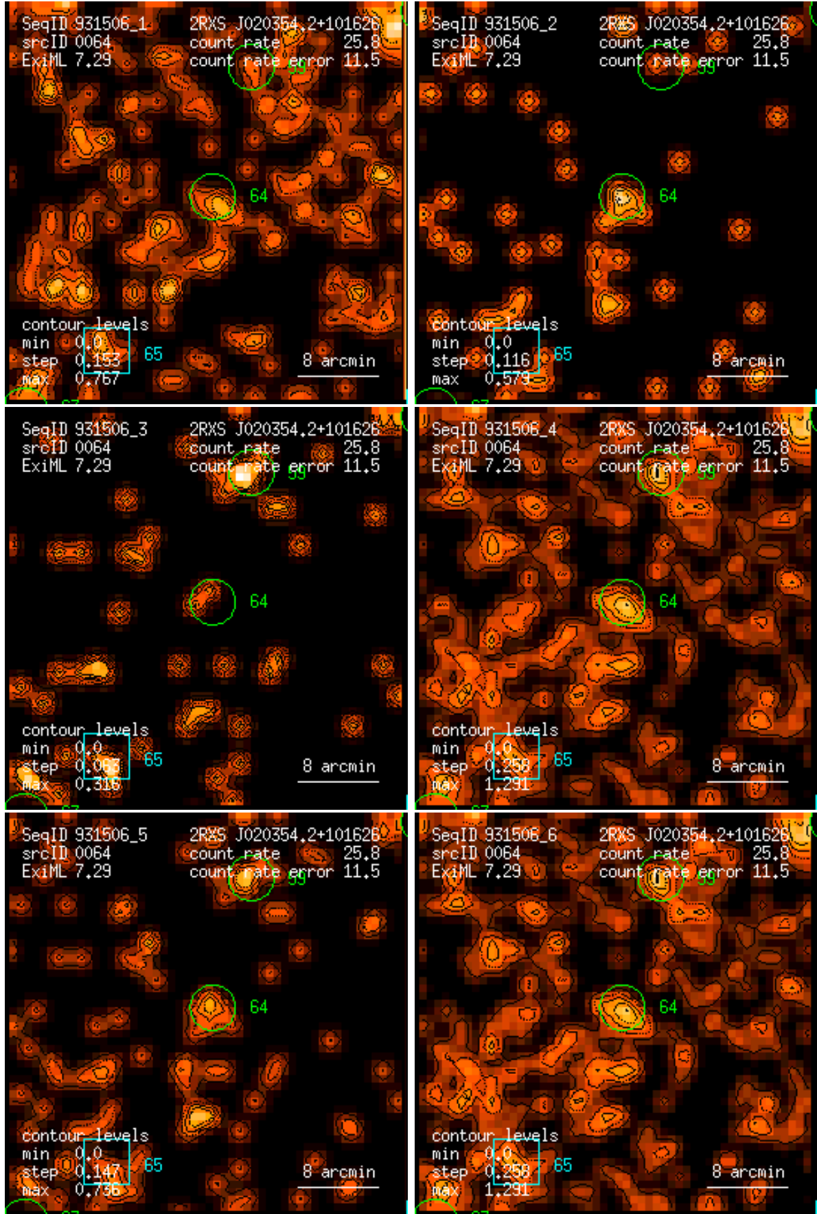
Figure 64: RASS 931506: detection 0064: band rate images, Gaussian filter: (1) PSPC channels 11 – 41, (2) 52 – 90, (3) 91 – 201, (4) 11 – 235, (5) 52 – 201, (6) 11 – 201. Broad band rates in counts/ks. Band rate contour levels in counts/ks/arcmin 2 .
