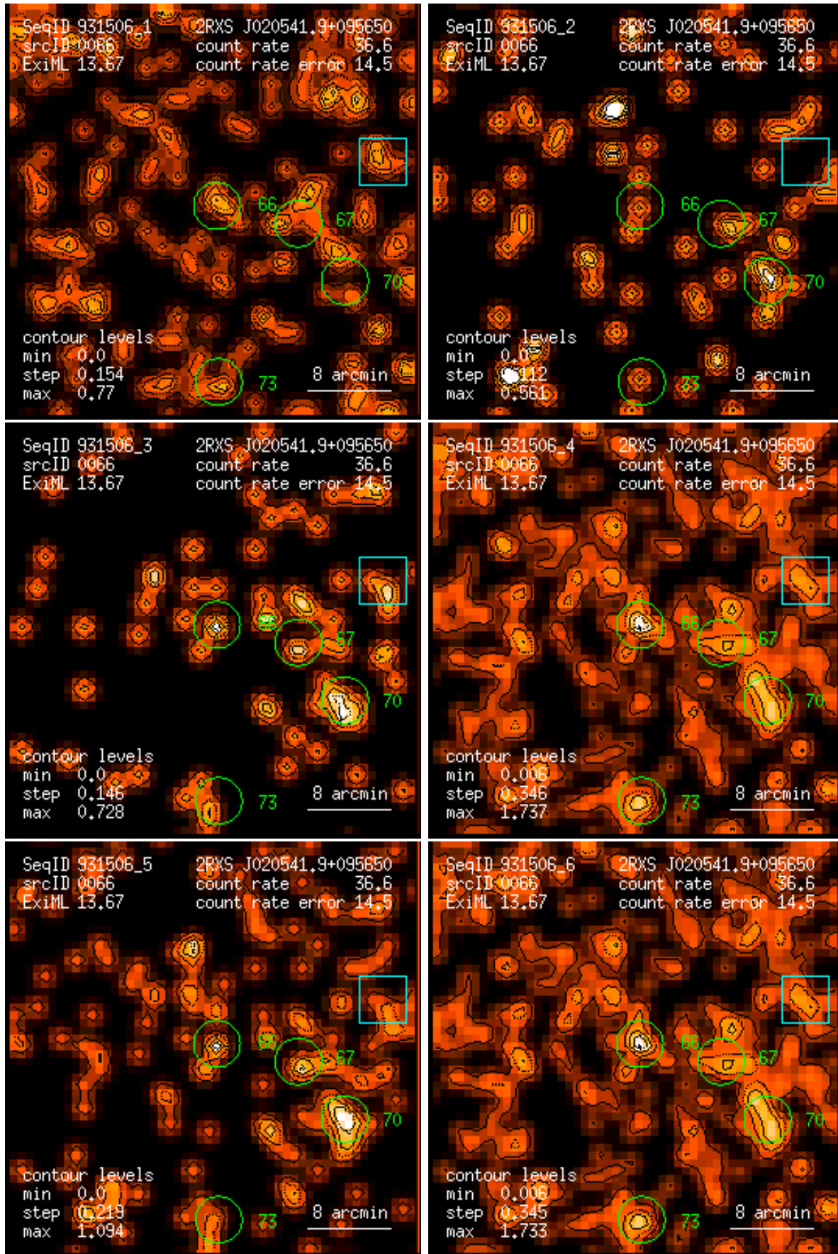
Figure 66: RASS 931506: detection 0066: band rate images, Gaussian filter: (1) PSPC channels 11 – 41, (2) 52 – 90, (3) 91 – 201, (4) 11 – 235, (5) 52 – 201, (6) 11 – 201. Broad band rates in counts/ks. Band rate contour levels in counts/ks/arcmin 2 .
