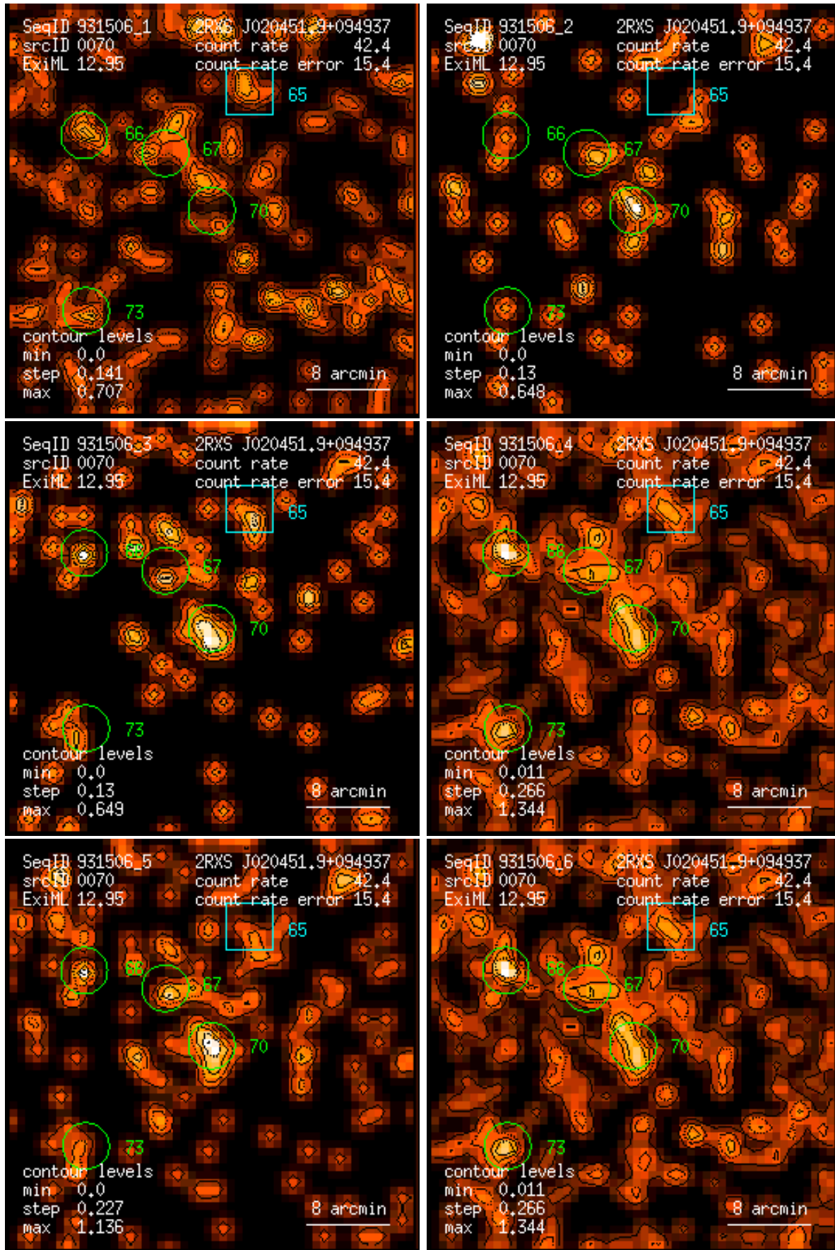
Figure 70: RASS 931506: detection 0070: band rate images, Gaussian filter: (1) PSPC channels 11 – 41, (2) 52 – 90, (3) 91 – 201, (4) 11 – 235, (5) 52 – 201, (6) 11 – 201. Broad band rates in counts/ks. Band rate contour levels in counts/ks/arcmin 2 .
