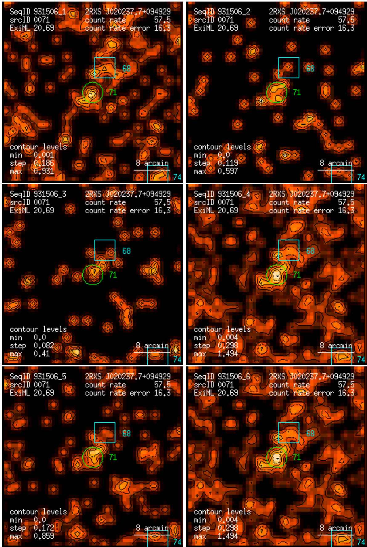
Figure 71: RASS 931506: detection 0071: band rate images, Gaussian filter: (1) PSPC channels 11 – 41, (2) 52 – 90, (3) 91 – 201, (4) 11 – 235, (5) 52 – 201, (6) 11 – 201. Broad band rates in counts/ks. Band rate contour levels in counts/ks/arcmin 2 .
