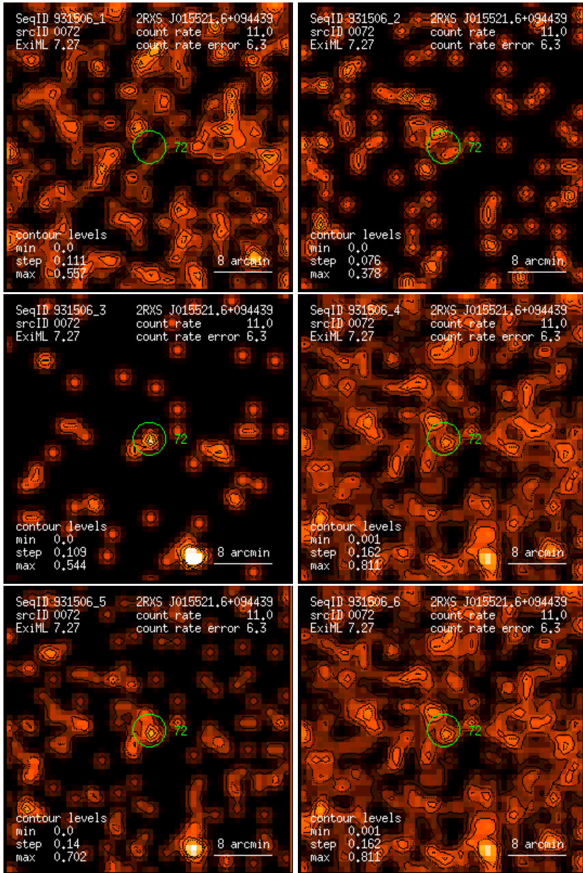
Figure 72: RASS 931506: detection 0072: band rate images, Gaussian filter: (1) PSPC channels 11 – 41, (2) 52 – 90, (3) 91 – 201, (4) 11 – 235, (5) 52 – 201, (6) 11 – 201. Broad band rates in counts/ks. Band rate contour levels in counts/ks/arcmin 2 .
