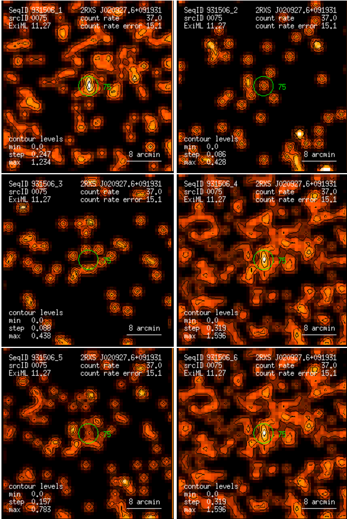
Figure 75: RASS 931506: detection 0075: band rate images, Gaussian filter: (1) PSPC channels 11 – 41, (2) 52 – 90, (3) 91 – 201, (4) 11 – 235, (5) 52 – 201, (6) 11 – 201. Broad band rates in counts/ks. Band rate contour levels in counts/ks/arcmin 2 .
