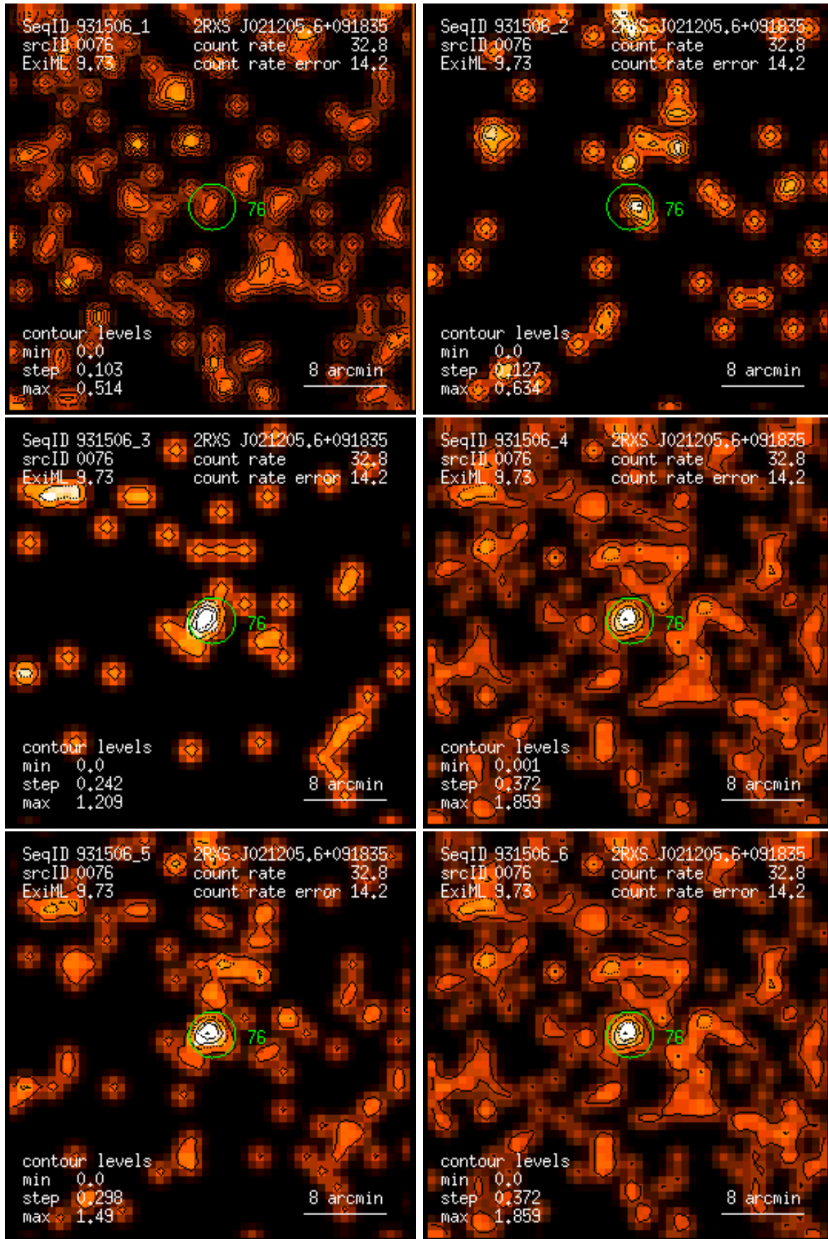
Figure 76: RASS 931506: detection 0076: band rate images, Gaussian filter: (1) PSPC channels 11 – 41, (2) 52 – 90, (3) 91 – 201, (4) 11 – 235, (5) 52 – 201, (6) 11 – 201. Broad band rates in counts/ks. Band rate contour levels in counts/ks/arcmin 2 .
